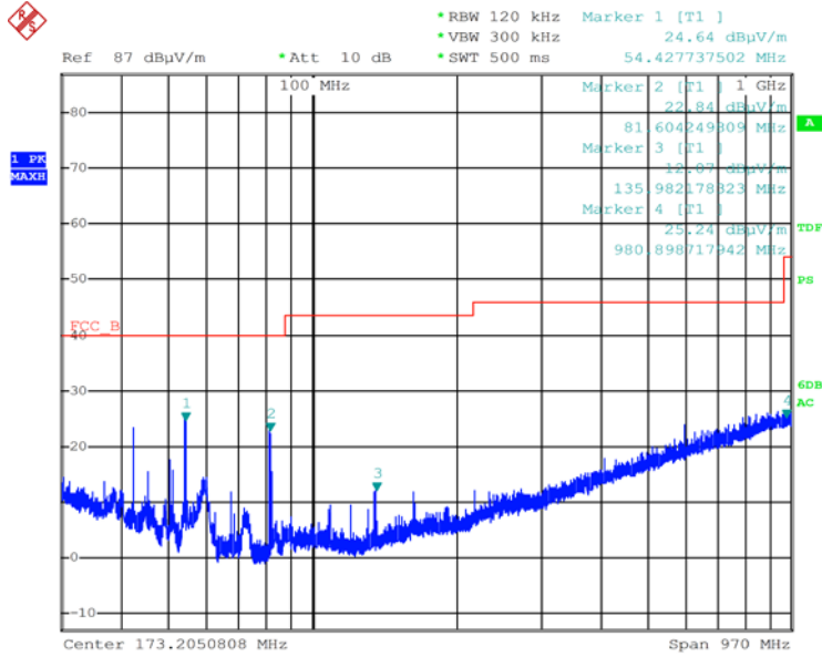
Radiated emissions (Below 1 000 MHz)
