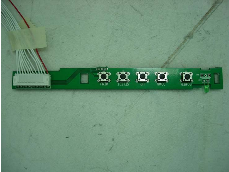
OSD Board ( Front )
