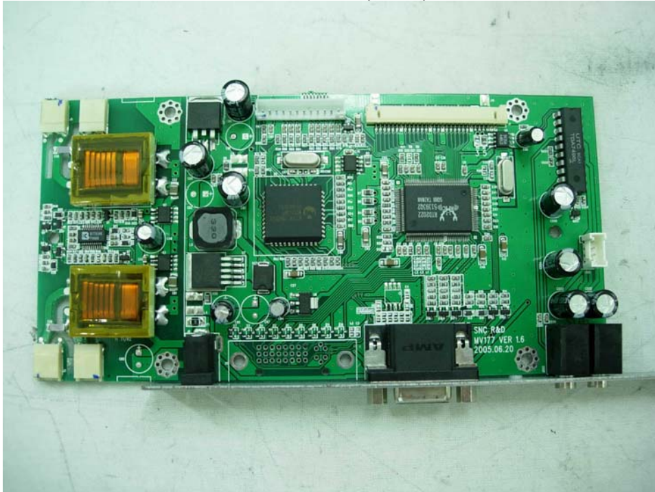
Main Controller ( Front )
