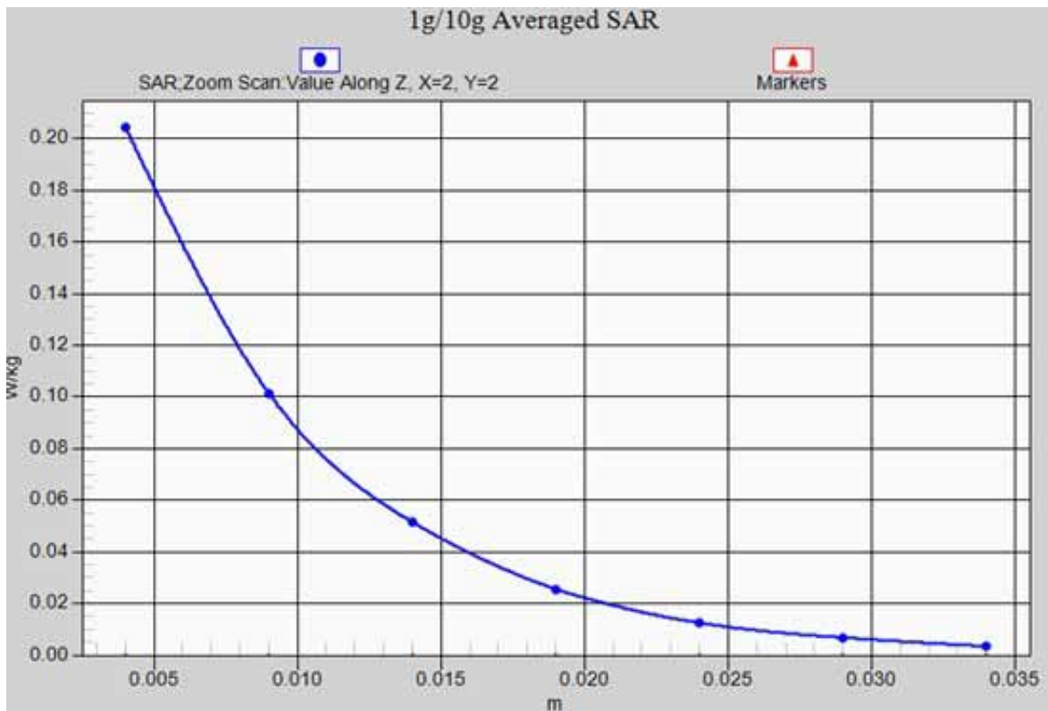
WiFi 802.11b(Body)/Back side-Low_ z-axis scan
