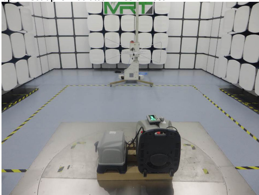
Photograph 2: Set-up for Radiated Emission Test
