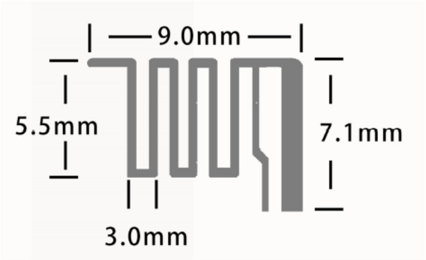
Match Network
