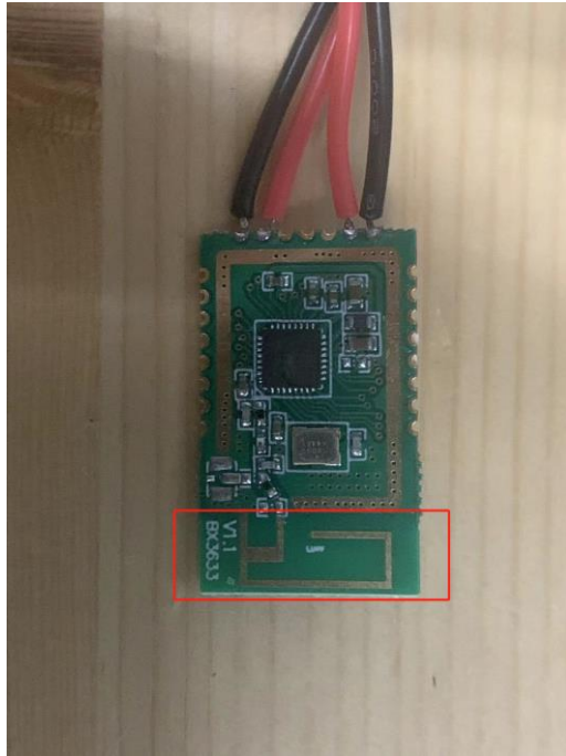
Antenna length: 10mm×4mm
