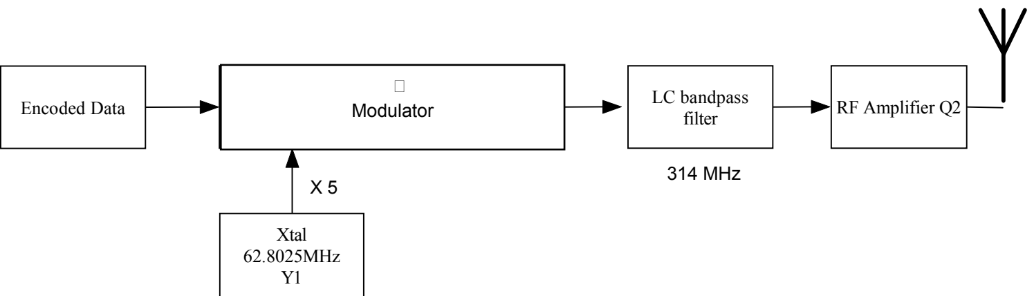
Block diagram of CED8000 RF module
