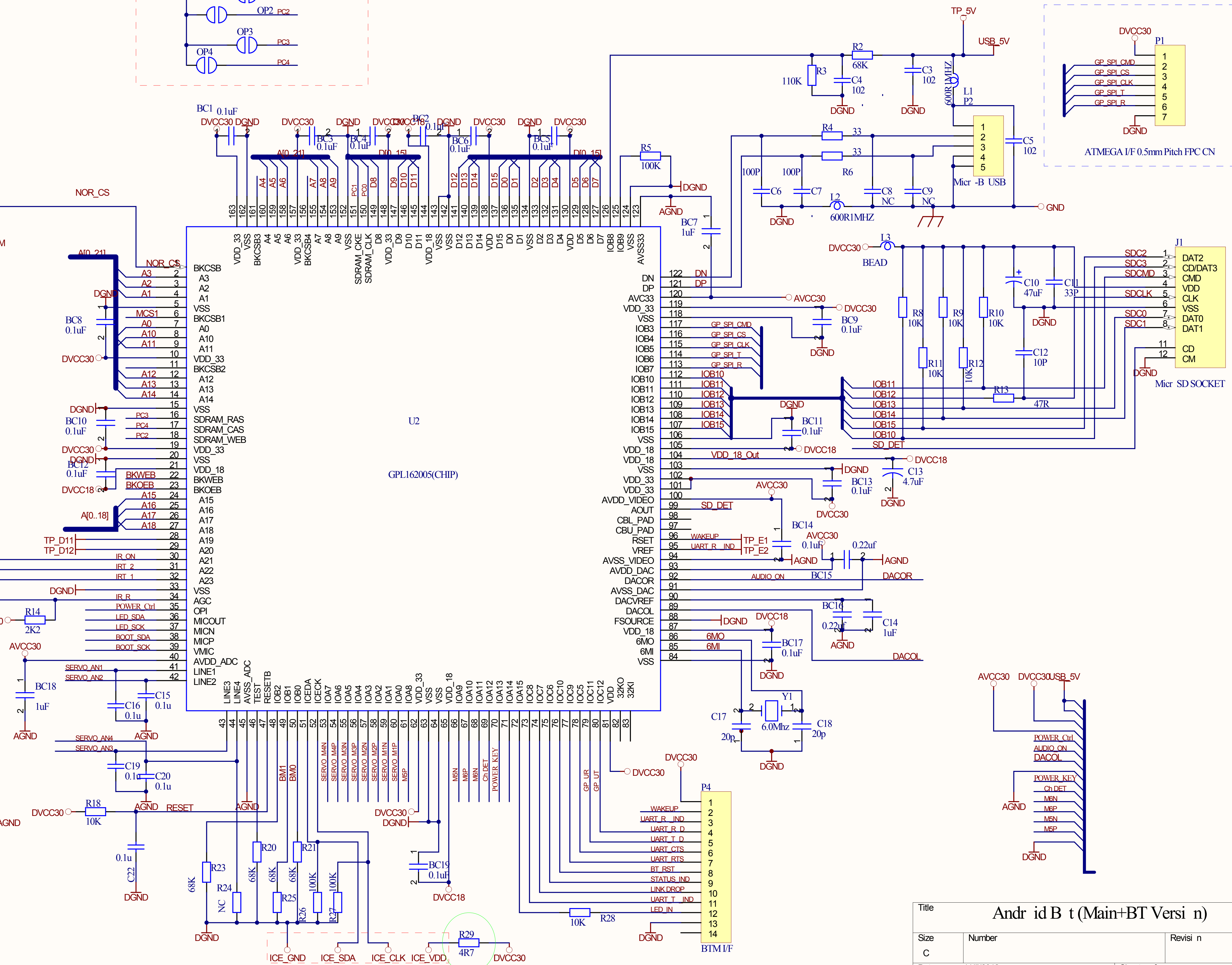
DEBUG PORT PAD
