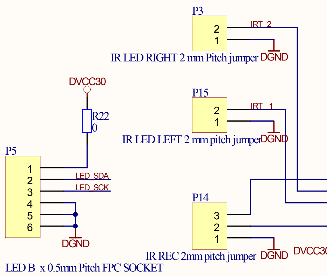
LED B x 0.5mm Pitch FPC SOCKET
