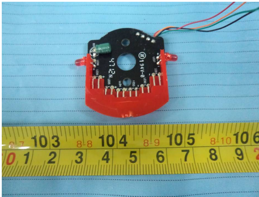
EUT – Head Board Bottom View
