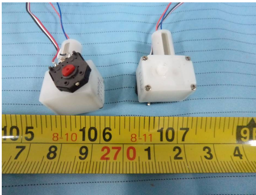
EUT – Arm Motors View
