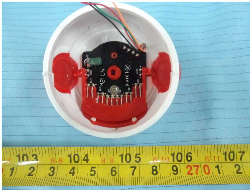
EUT – Head Board Full View
