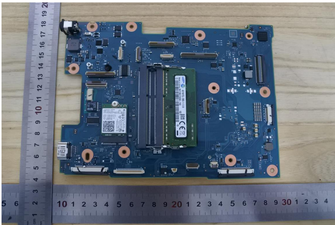
Internal View of EUT-24
