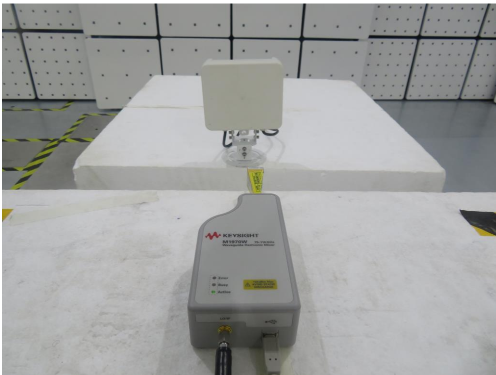
Description: Radiated Emission Test Setup for 75GHz ~100GHz (at 0.25m)
