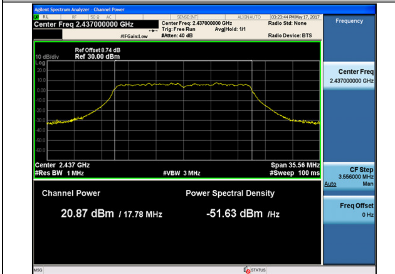
Maximum peak conducted output power_11N20SISO_2462_Ant1
