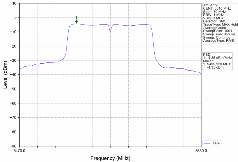
802.11ac(VHT40)_LCH_5510MHz_MIMO_NTNV
