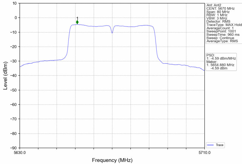
802.11ac(VHT40)_HCH_5670MHz_MIMO_NTNV
