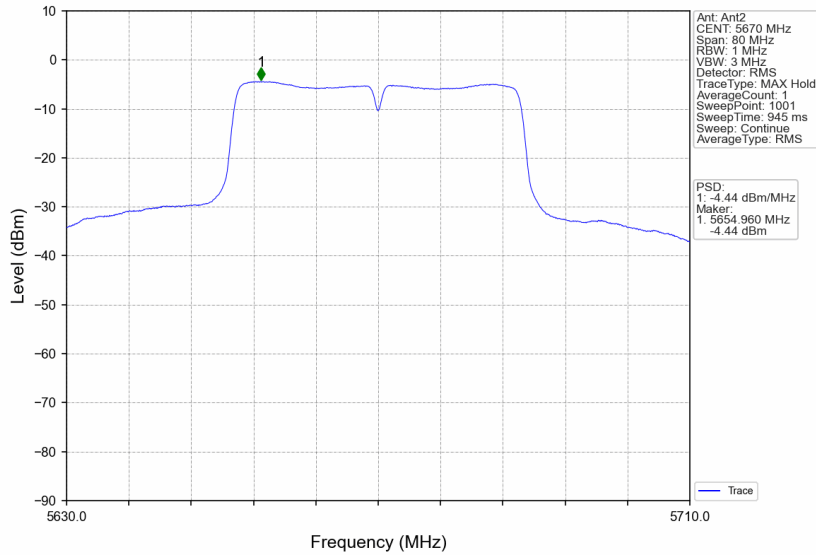
802.11n(HT40)_HCH_5670MHz_MIMO_NTNV
