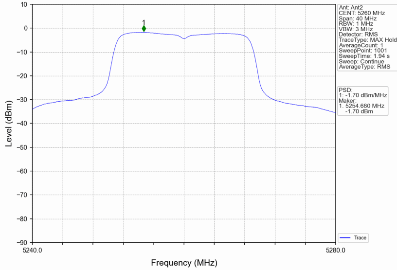
802.11ac(VHT20)_LCH_5260MHz_MIMO_NTNV
