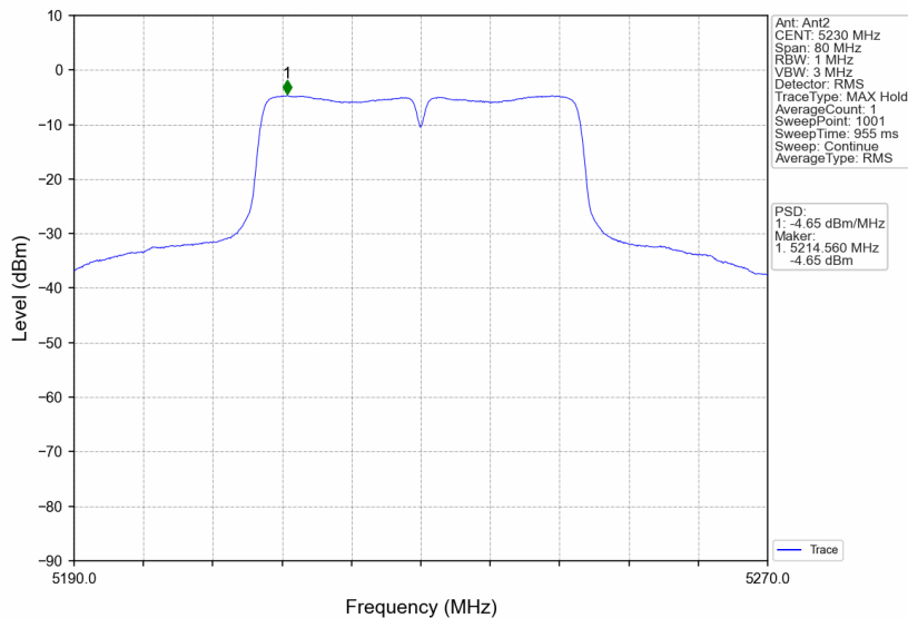
802.11ac(VHT40)_HCH_5230MHz_Ant2_NTNV
