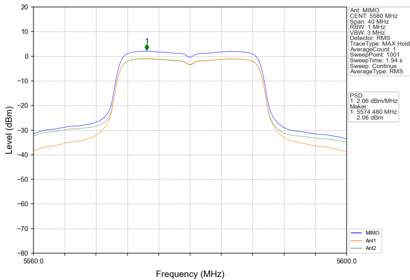
802.11ac(VHT20)_MCH_5580MHz_MIMO_NTNV
