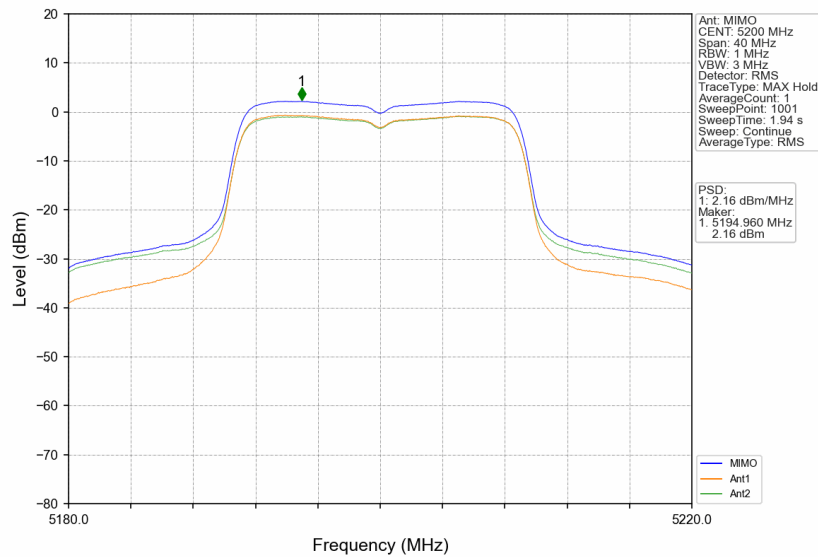
802.11ac(VHT20)_MCH_5200MHz_MIMO_NTNV
