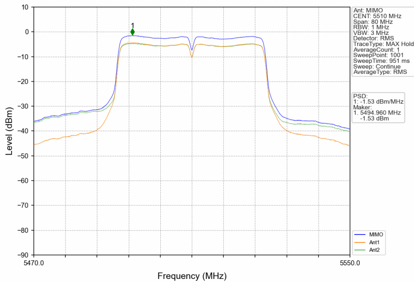
802.11n(HT40)_LCH_5510MHz_MIMO_NTNV
