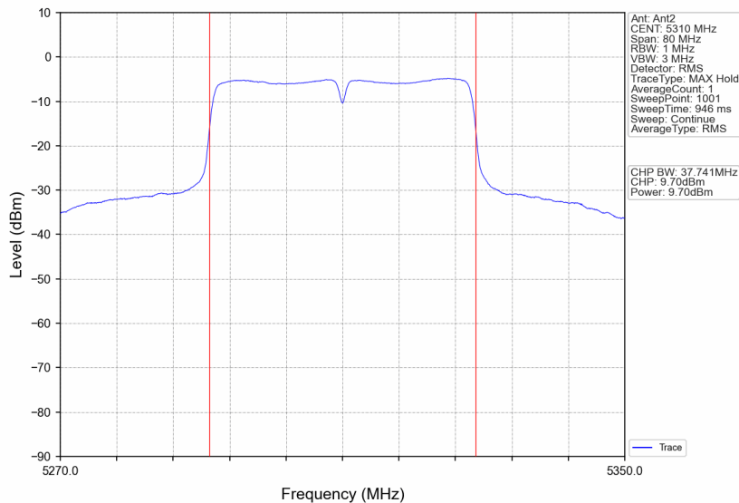
802.11n(HT40)_HCH_5310MHz_Ant2_NTNV
