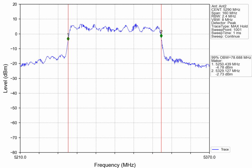
802.11ac(VHT80)_MCH_5290MHz_Ant2_NTNV
