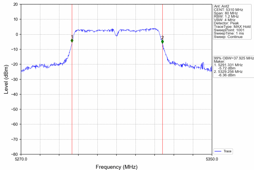
802.11ac(VHT40)_HCH_5310MHz_Ant2_NTNV
