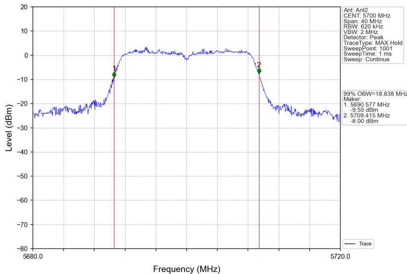
802.11ac(VHT20)_HCH_5700MHz_Ant2_NTNV
