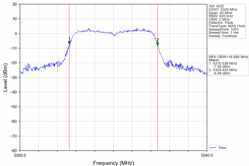
802.11ac(VHT20)_HCH_5320MHz_Ant2_NTNV
