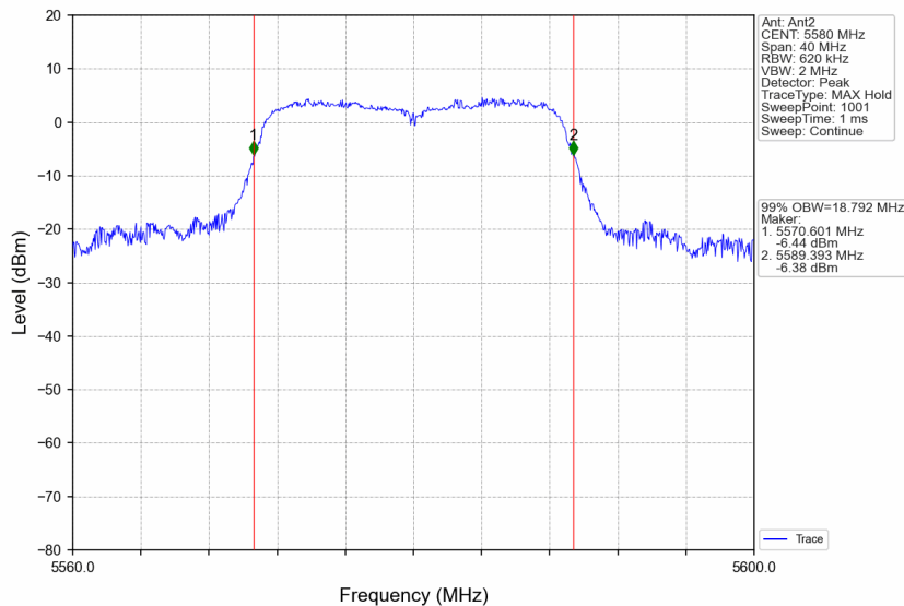
802.11ac(VHT20)_MCH_5580MHz_Ant2_NTNV
