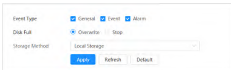
Figure 6-13 Local storage
