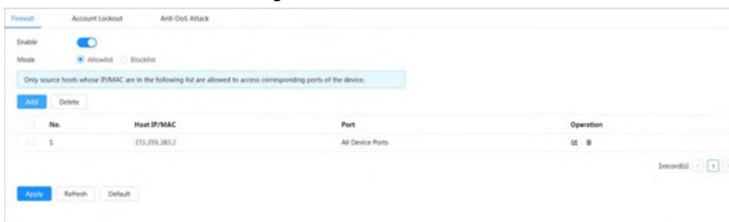
Figure 9-6 Firewall
