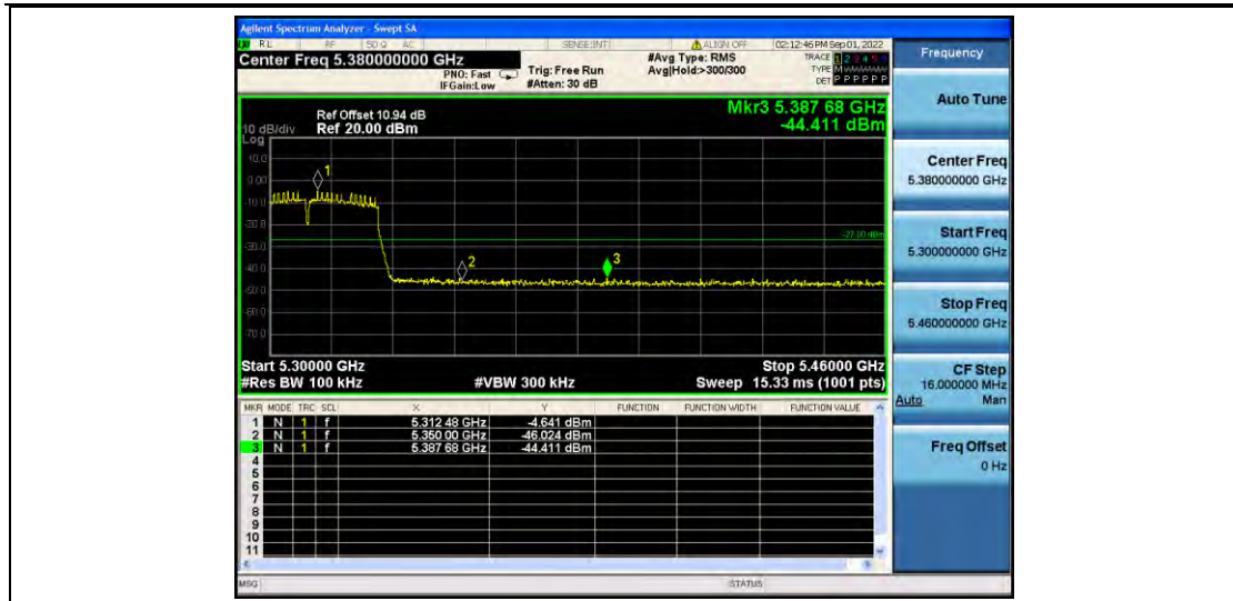
11AC40MIMO_Ant2_High_5310
