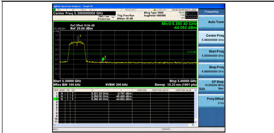
11AC20MIMO_Ant2_High_5320
