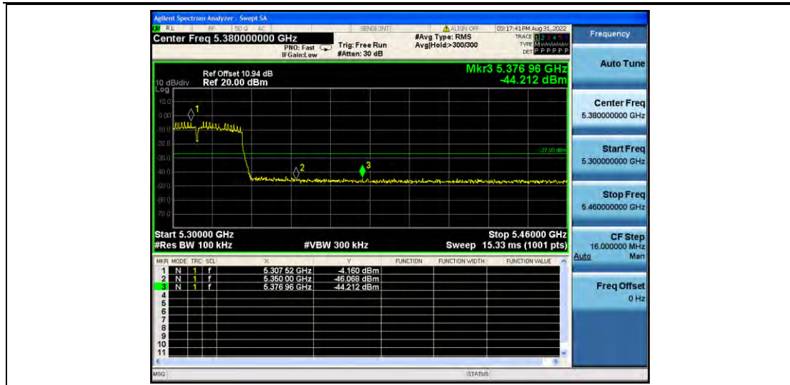
11N40MIMO_Ant2_High_5310
