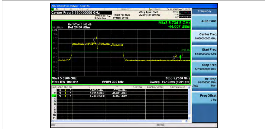
11AC80MIMO_Ant2_High_5610
