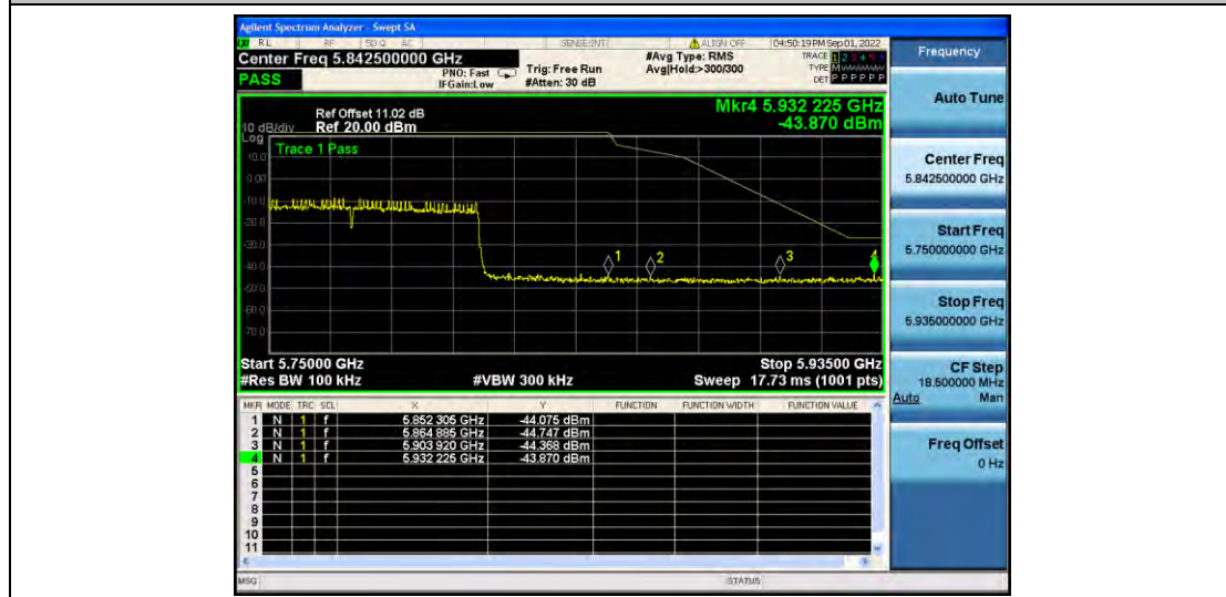
11AC80MIMO_Ant2_High_5775
