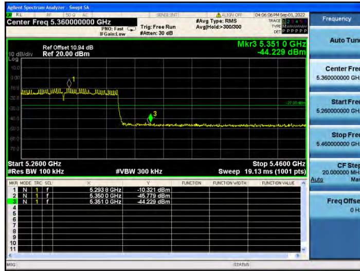
11AC80MIMO_Ant2_High_5290
