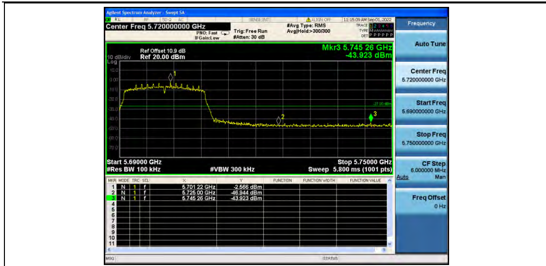
11AC20MIMO_Ant2_High_5700
