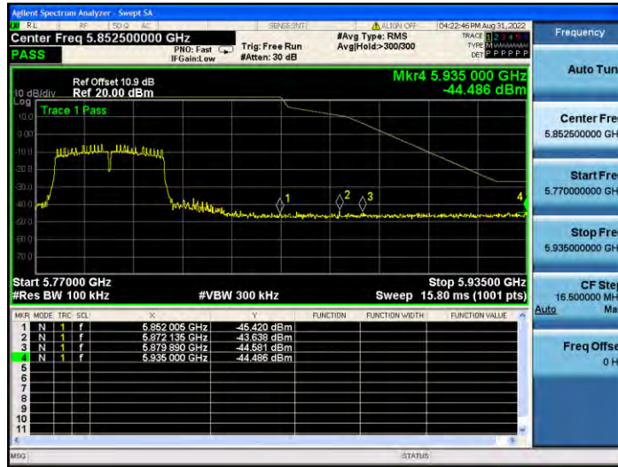
11N40MIMO_Ant2_High_5795
