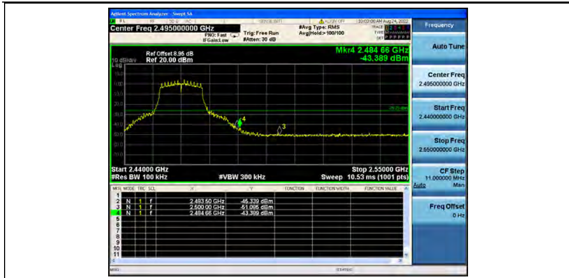
11G_Ant2_High_2462
