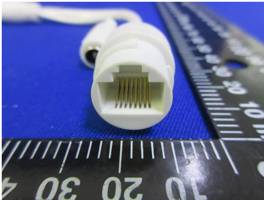
RJ45 Port
