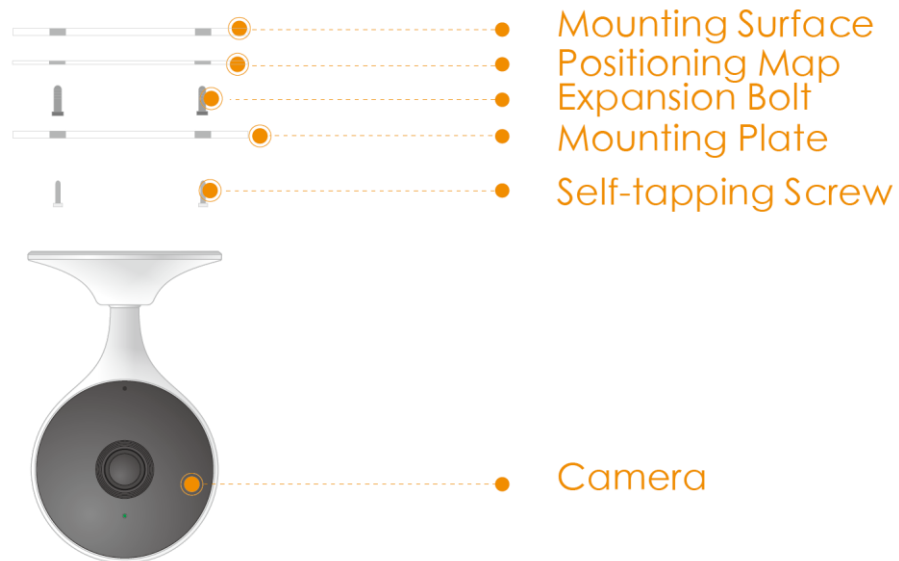
Figure 4-1 Installation diagram
