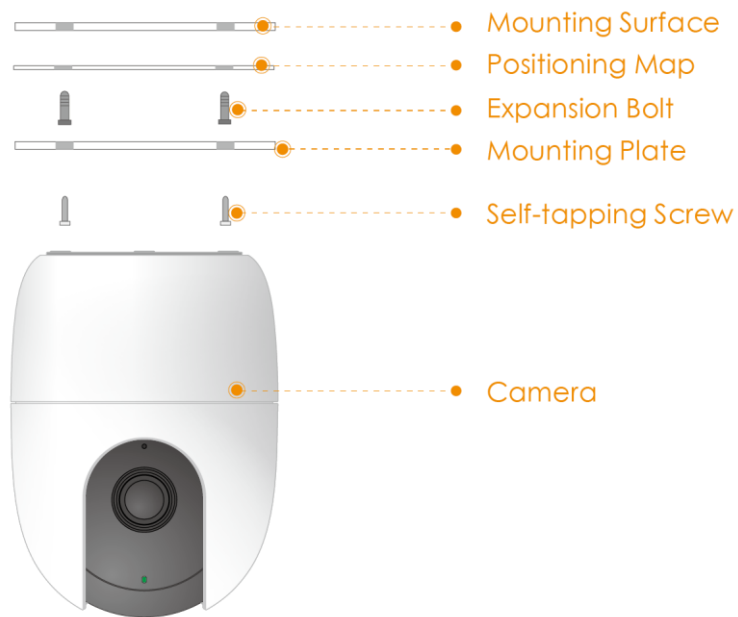
Figure 4-1 Installation diagram
