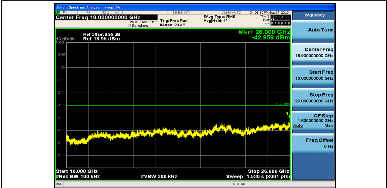
RF Conducted Spurious Emissions_11N20SISO_2462
