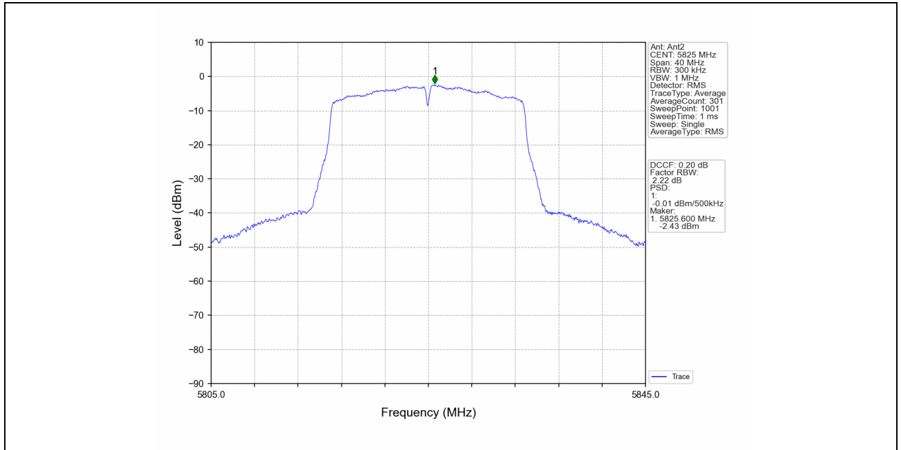
802.11ac(VHT20)_HCH_5825MHz_MIMO_NTNV
