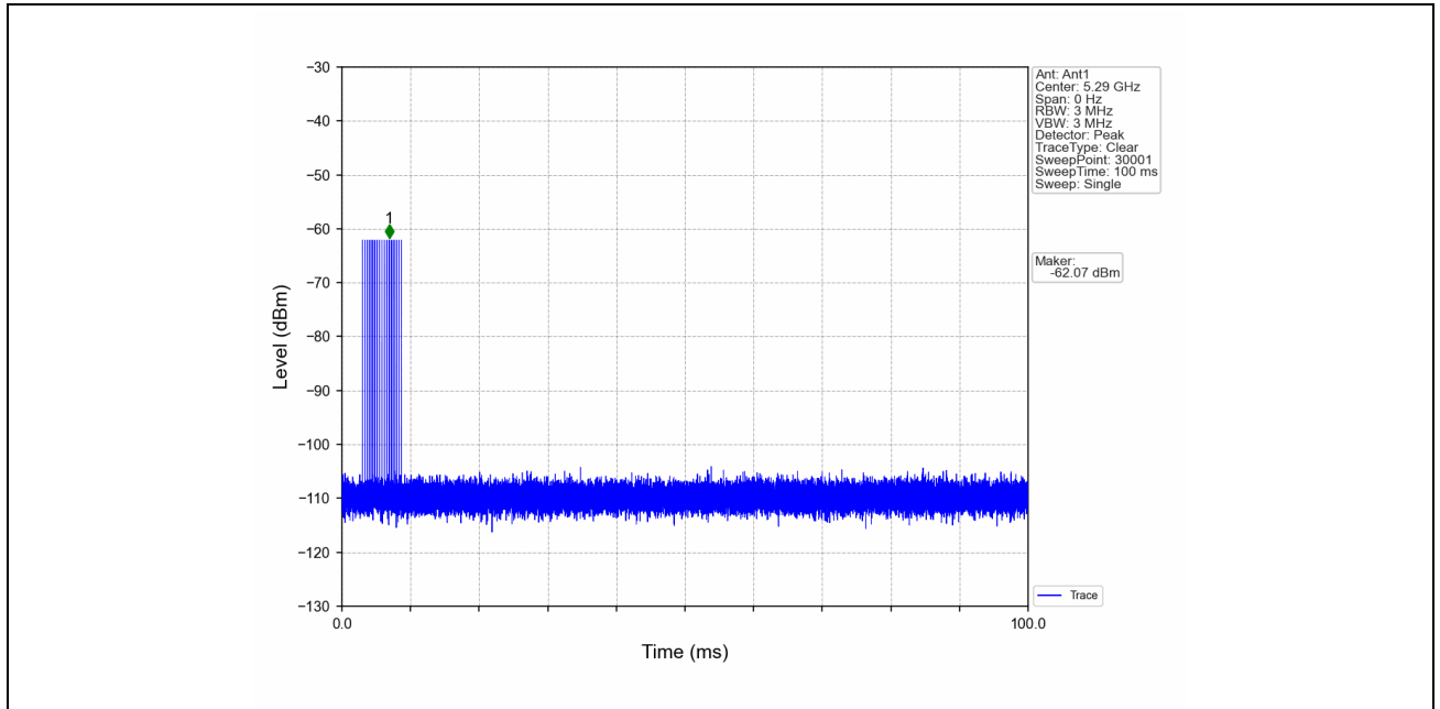
Signal Calibration_802.11ac(VHT80)_2A_5290MHz_RadarType4_Trial0
