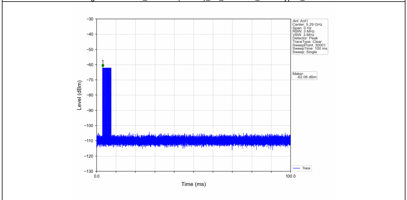
Signal Calibration_802.11ac(VHT80)_2A_5290MHz_RadarType3_Trial0
