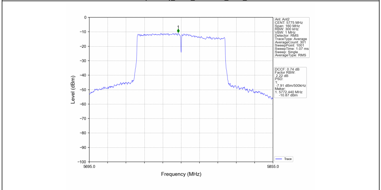
802.11ac(VHT80)_MCH_5775MHz_MIMO_NTNV
