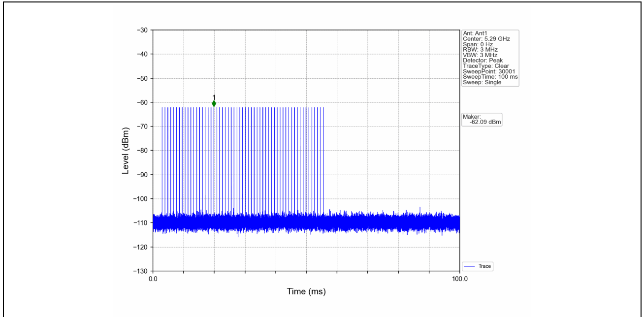
Signal Calibration_802.11ac(VHT80)_2A_5290MHz_RadarType2_Trial0
