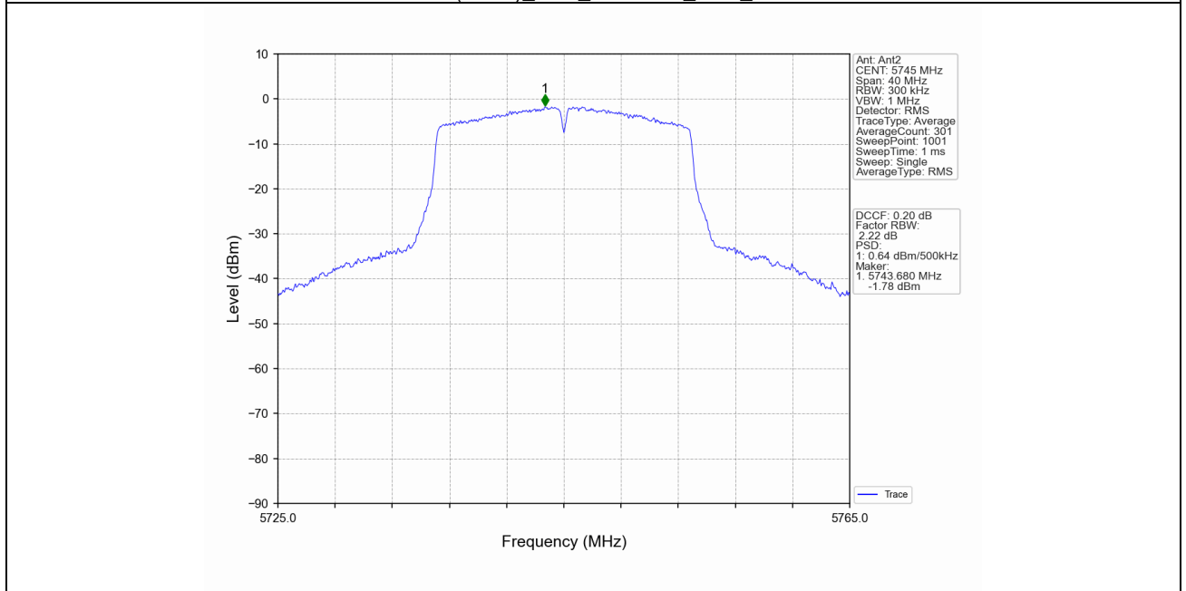
802.11n(HT20)_LCH_5745MHz_MIMO_NTNV
