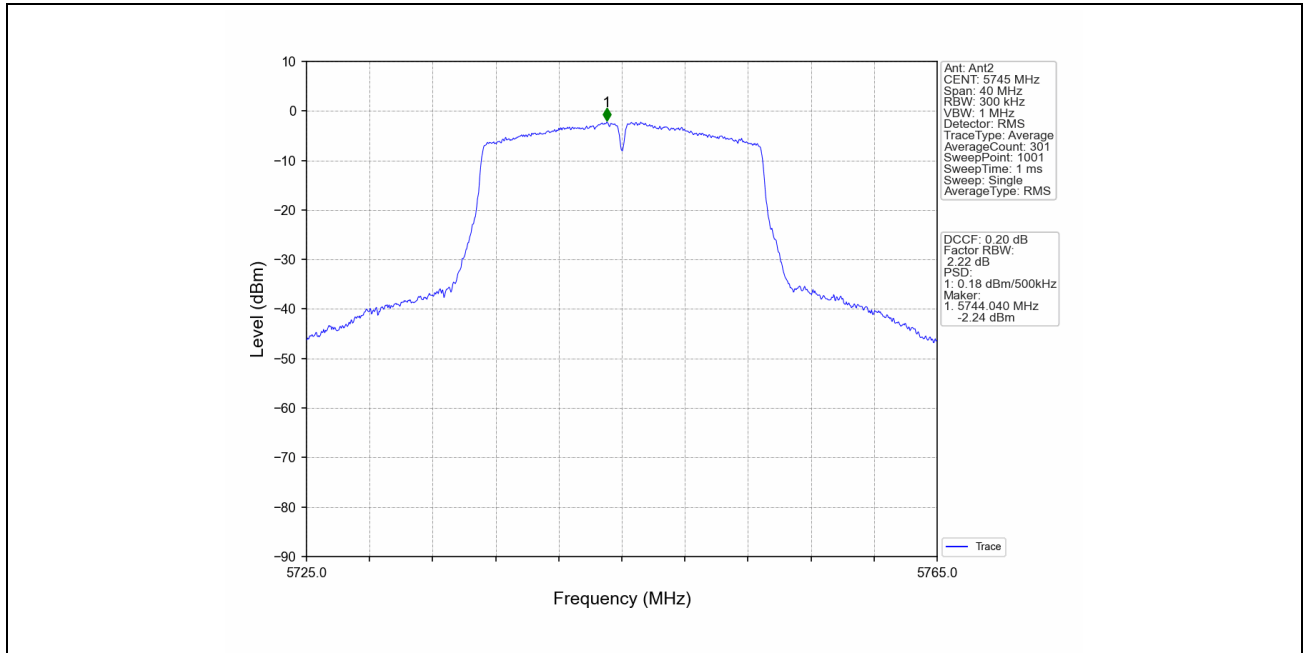
802.11ac(VHT20)_LCH_5745MHz_MIMO_NTNV
