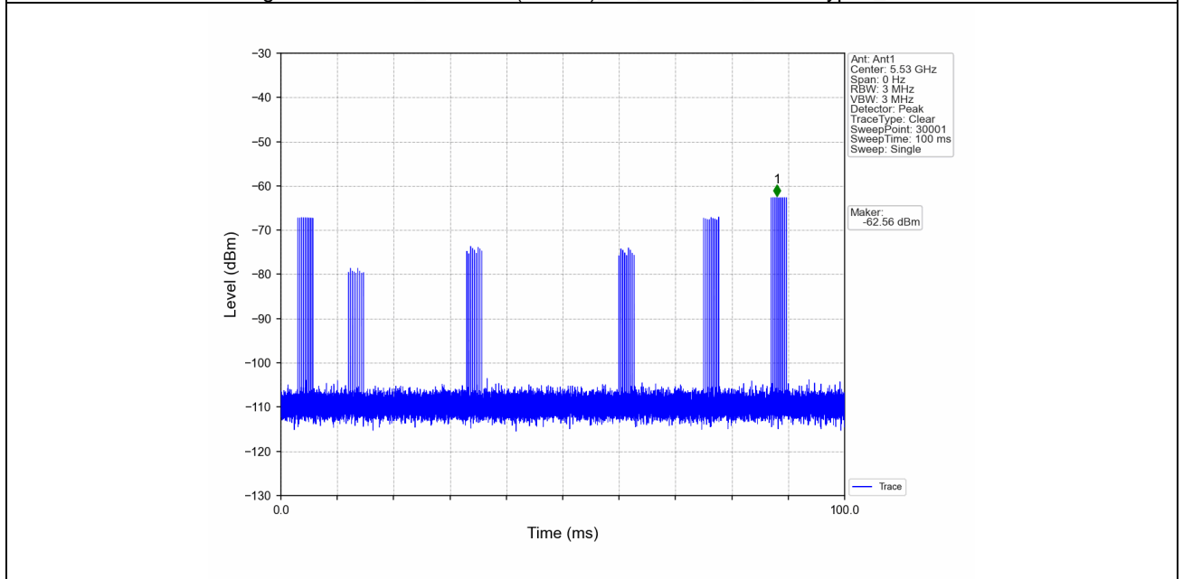
Signal Calibration_802.11ac(VHT80)_2C_5530MHz_RadarType6_Trial0
