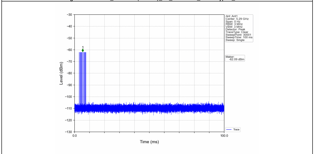
Signal Calibration_802.11ac(VHT80)_2A_5290MHz_RadarType5_Trial0
