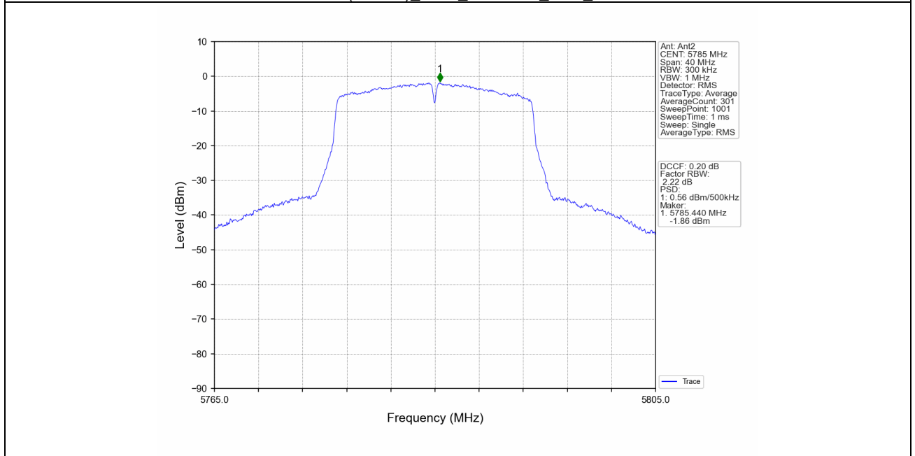
802.11ac(VHT20)_MCH_5785MHz_MIMO_NTNV
