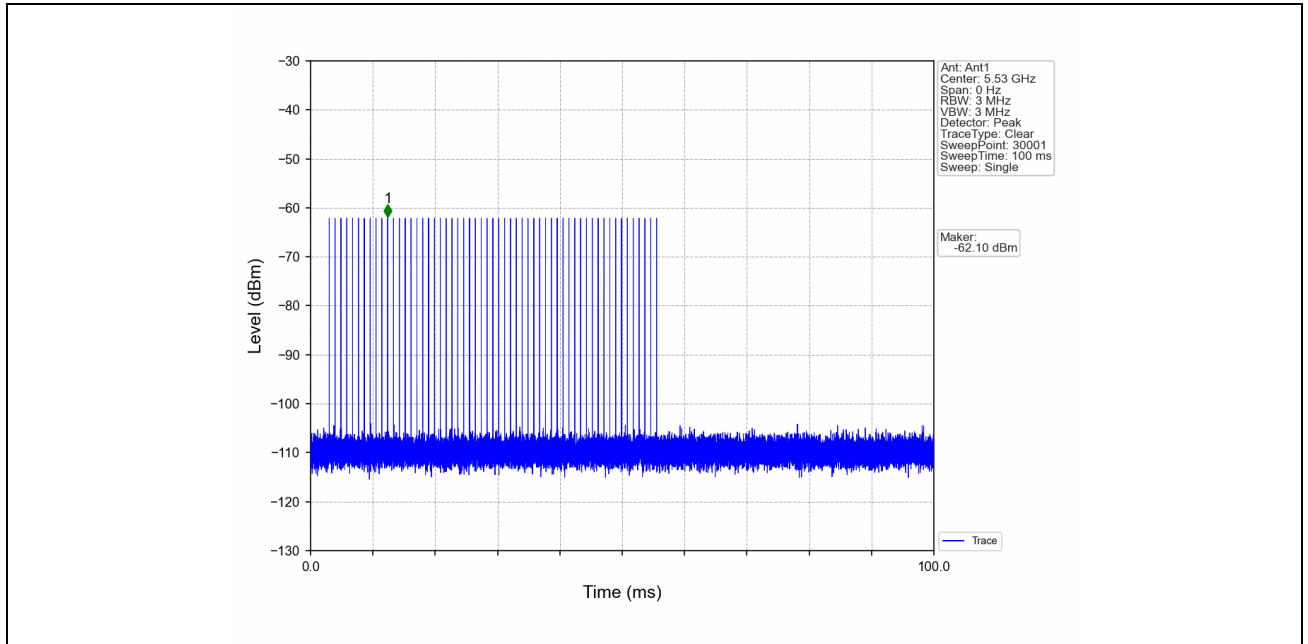
Signal Calibration_802.11ac(VHT80)_2C_5530MHz_RadarType2_Trial0
