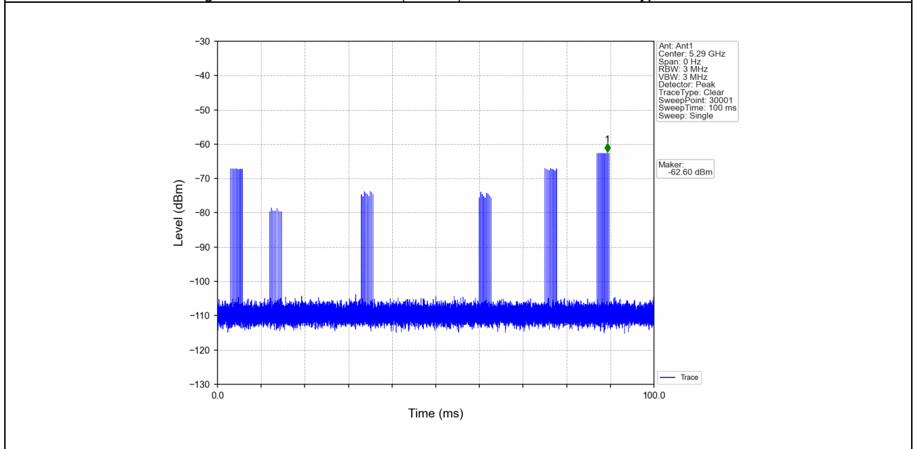
Signal Calibration_802.11ac(VHT80)_2A_5290MHz_RadarType6_Trial0
