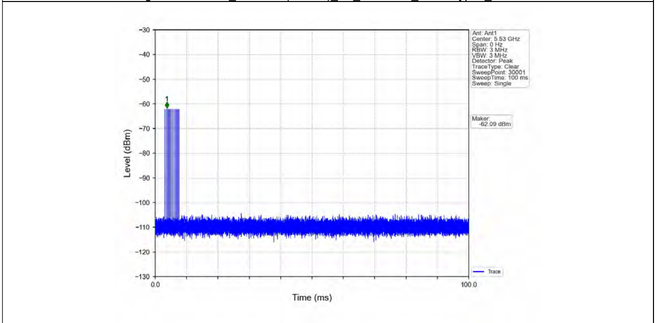
Signal Calibration_802.11ac(VHT80)_2C_5530MHz_RadarType5_Trial0
