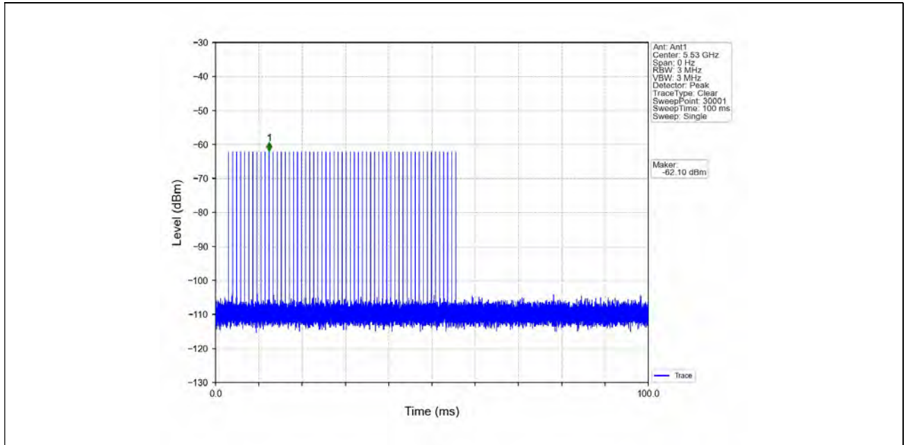
Signal Calibration_802.11ac(VHT80)_2C_5530MHz_RadarType2_Trial0
