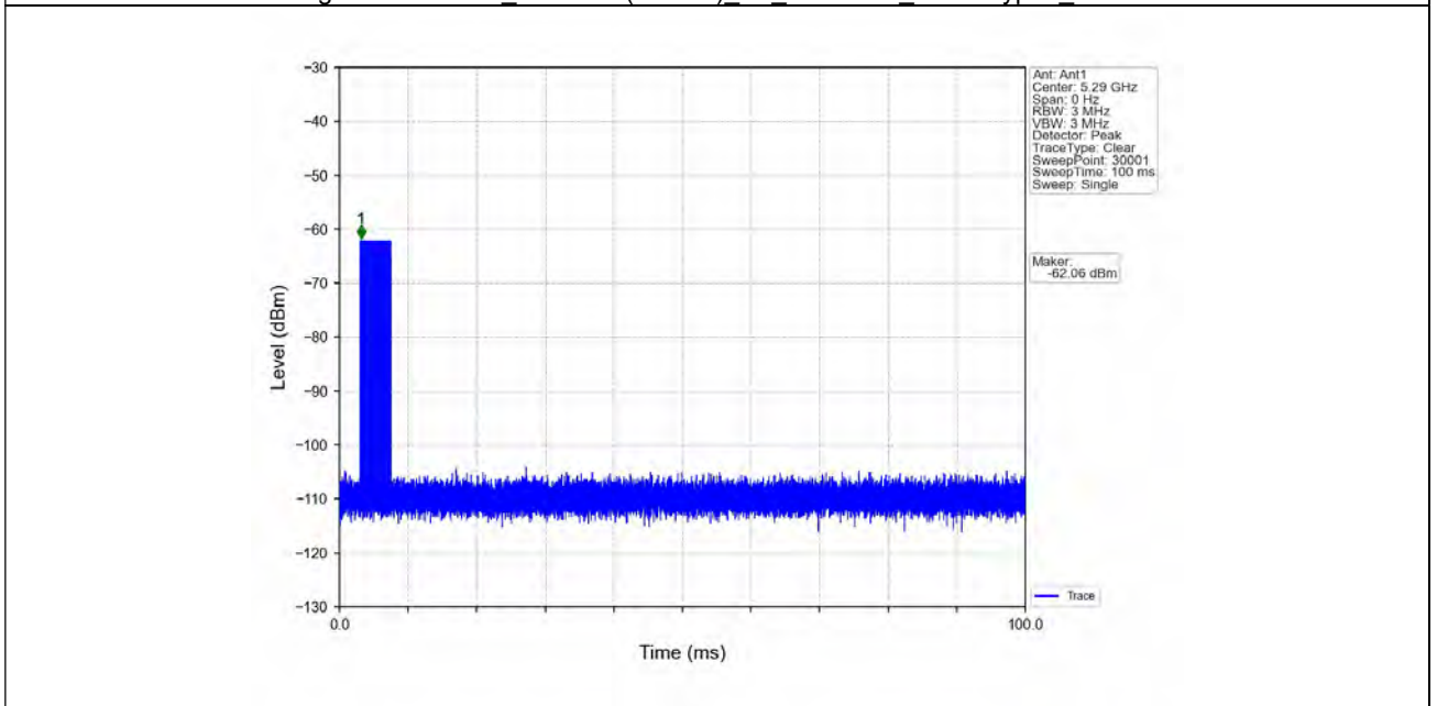
Signal Calibration 802.11ac(VHT80)_2A_5290MHz_RadarType3_Trial0
