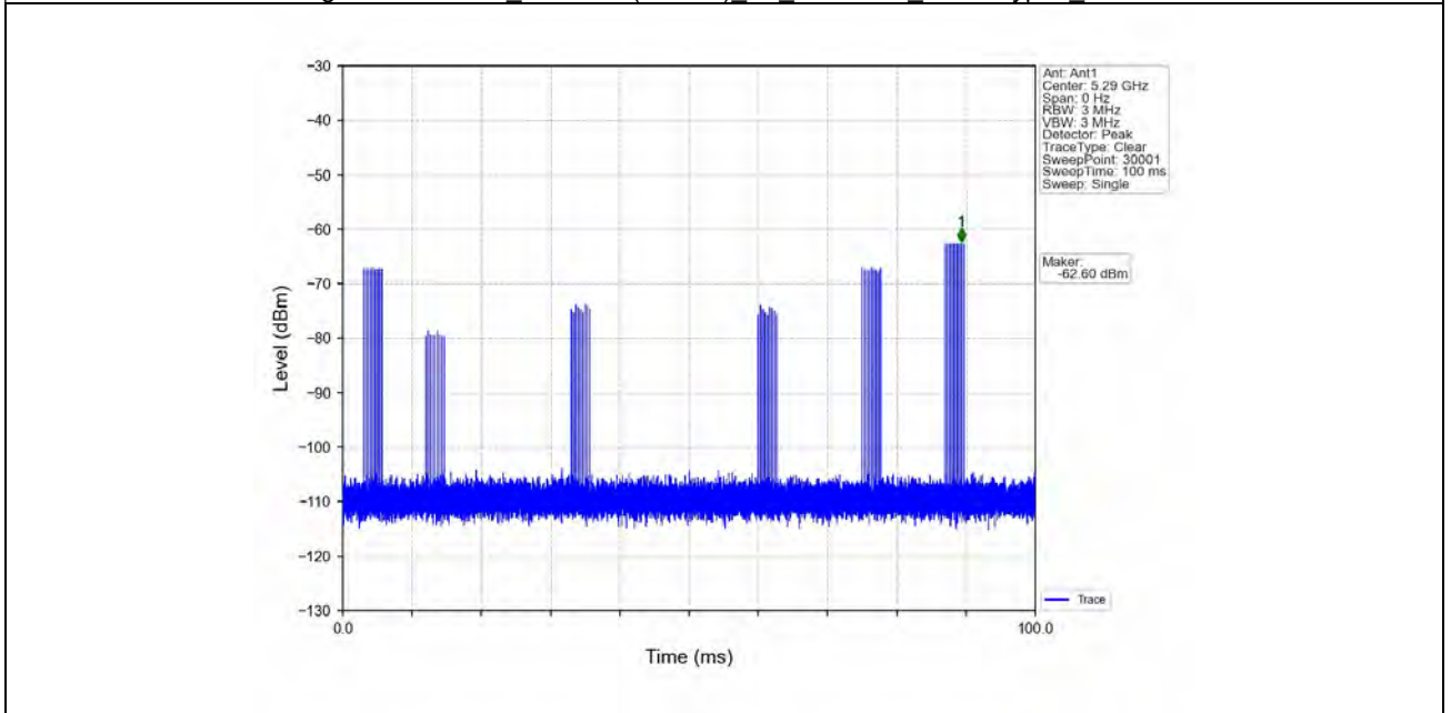
Signal Calibration_802.11ac(VHT80)_2A_5290MHz_RadarType6_Trial0
