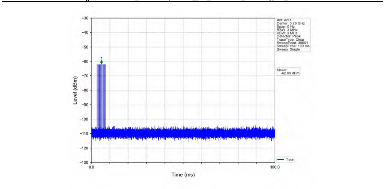
Signal Calibration 802.11ac(VHT80)_2A_5290MHz_RadarType5_Trial0
