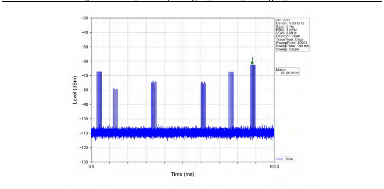
Signal Calibration_802.11ac(VHT80)_2C_5530MHz_RadarType6_Trial0
