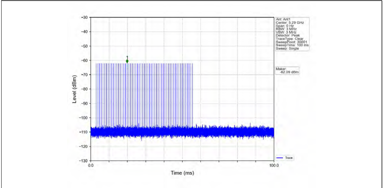
Signal Calibration 802.11ac(VHT80)_2A_5290MHz_RadarType2_Trial0
