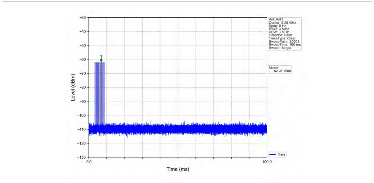
Signal Calibration 802.11ac(VHT80)_2A_5290MHz_RadarType4_Trial0
