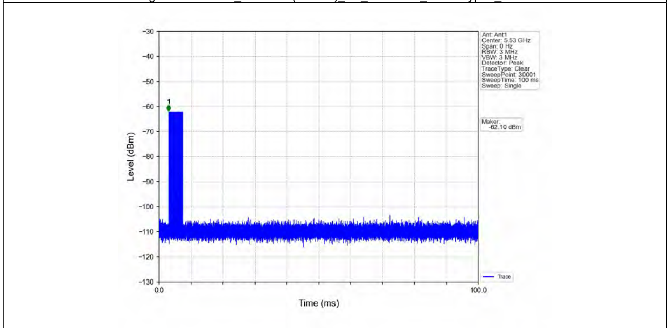
Signal Calibration_802.11ac(VHT80)_2C_5530MHz_RadarType3_Trial0
