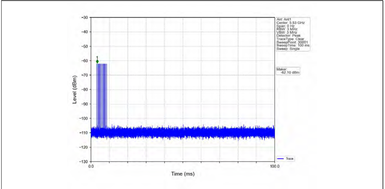
Signal Calibration_802.11ac(VHT80)_2C_5530MHz_RadarType4_Trial0
