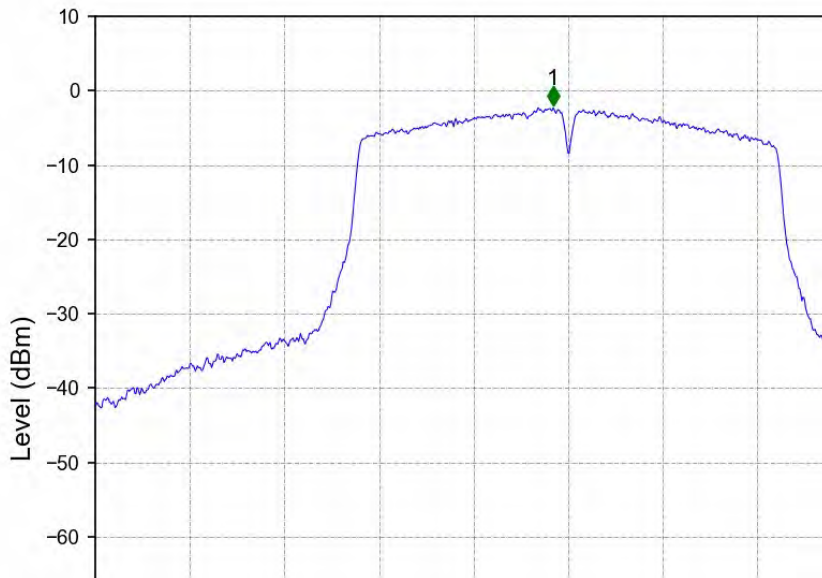
802.11n(HT20)_MCH_5785MHz_Ant2_NTNV
