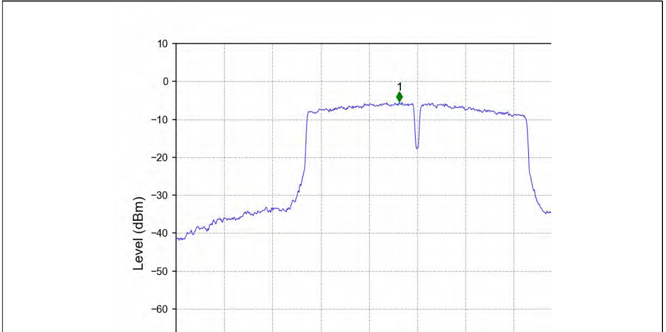
802.11ac(VHT40) HCH_5795MHz_MIMO_NTNV
