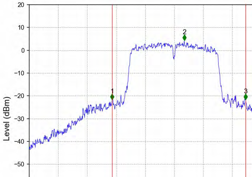
802.11ac(VHT40)_HCH_5310MHz_Ant2_NTNV
