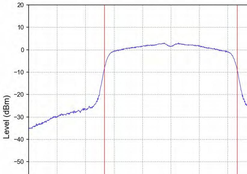
802.11ac(VHT20) LCH_5745MHz_Ant1_NTNV
