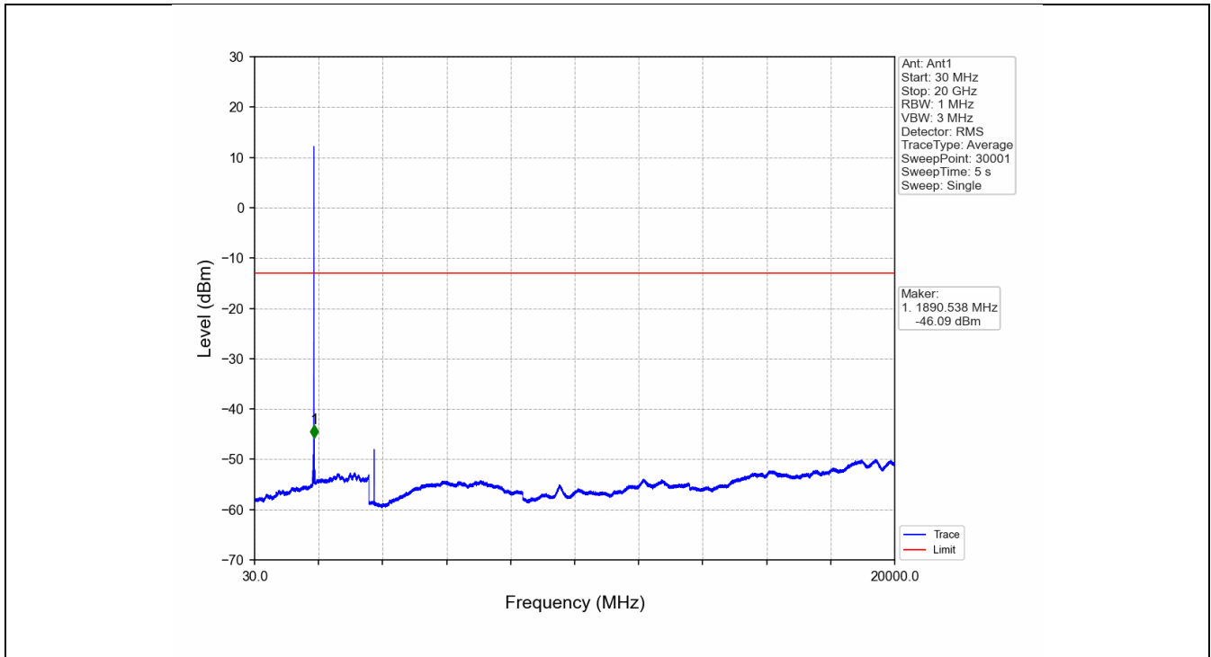
Band2_HSDPA_HCH_1907.6MHz_Subtest 1_NTNV
