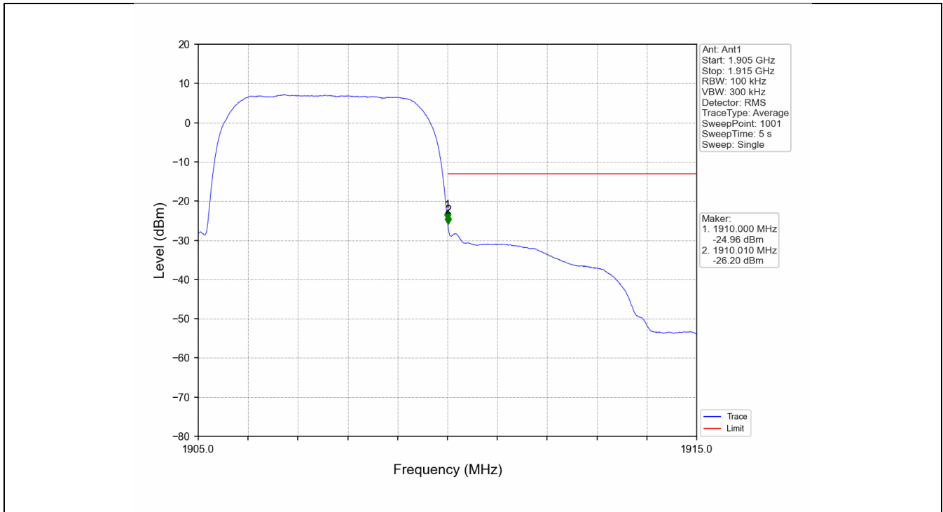
Band2_RMC_HCH_1907.6MHz_12.2kbps RMC_NTNV
