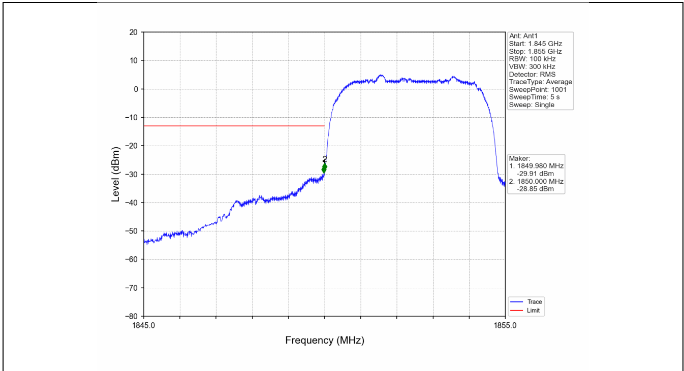
Band2_HSDPA_LCH_1852.4MHz_Subtest 1_NTNV
