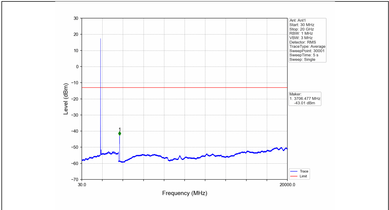
Band2_RMC_MCH_1880MHz_12.2kbps RMC_NTNV
