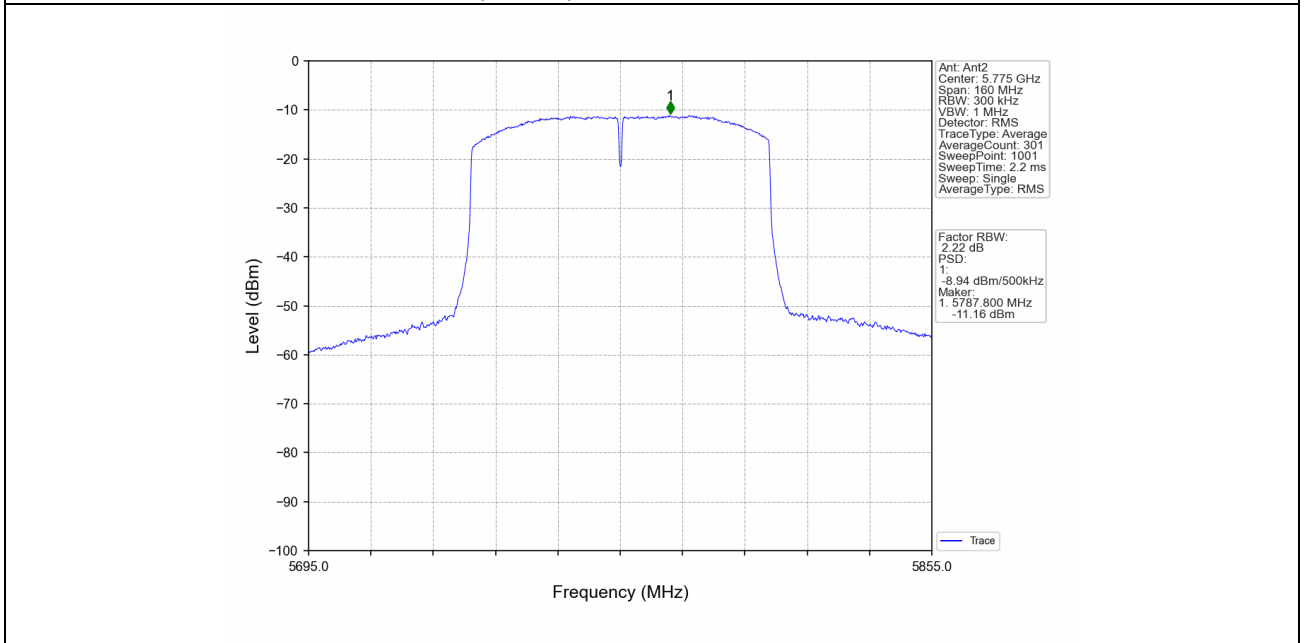
802.11ac(VHT80)_MCH_5775MHz_MIMO_NTNV
