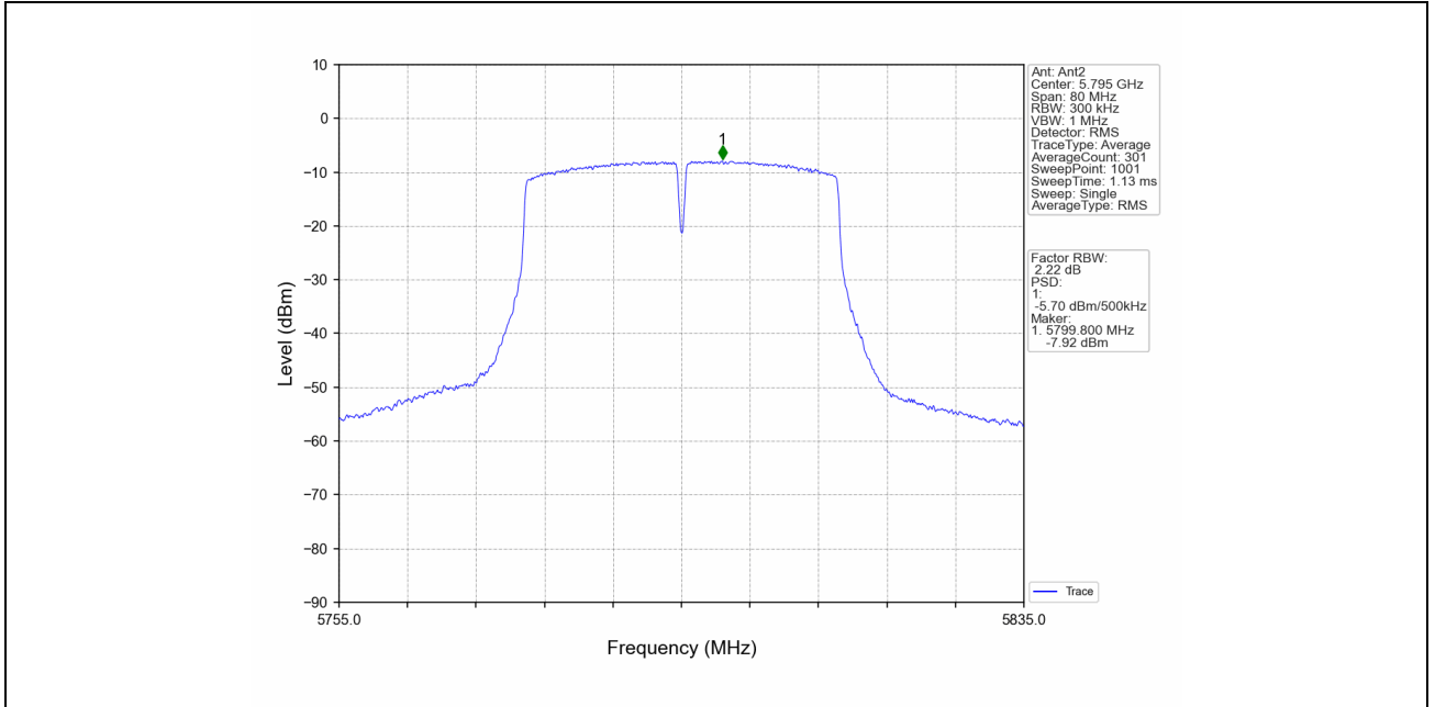
802.11ac(VHT40)_HCH_5795MHz_MIMO_NTNV
