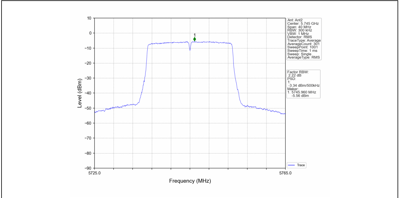
802.11ac(VHT20)_LCH_5745MHz_MIMO_NTNV
