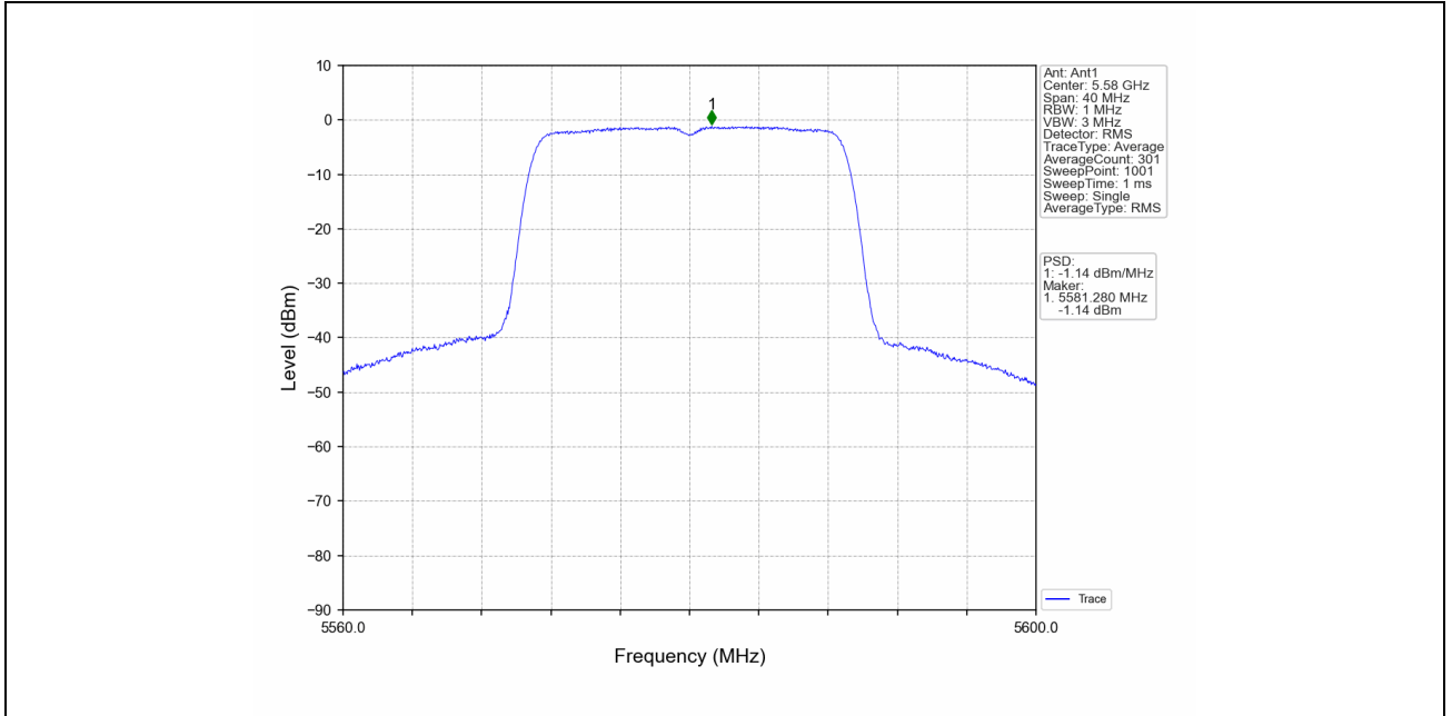
802.11ac(VHT20)_MCH_5580MHz_Ant2_NTNV
