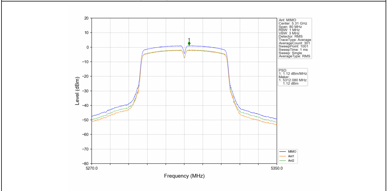
802.11ac(VHT40)_LCH_5310MHz_Ant1_NTNV
