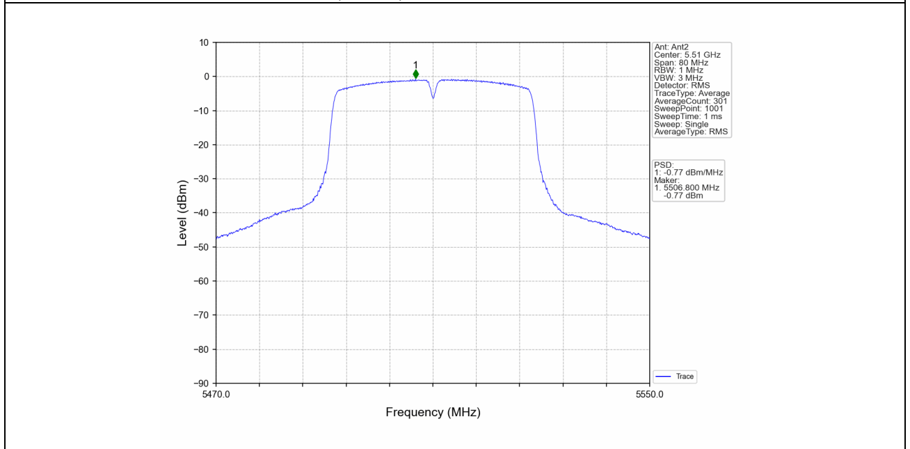
802.11ac(VHT40)_LCH_5510MHz_MIMO_NTNV
