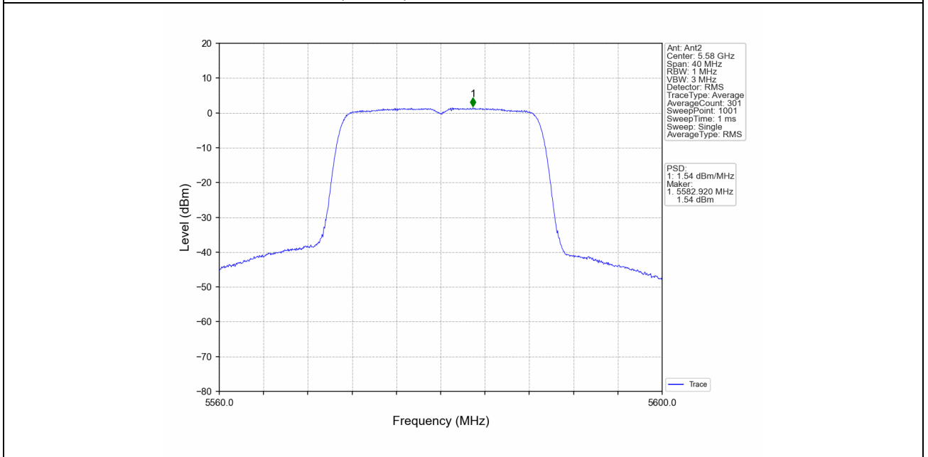
802.11ac(VHT20)_MCH_5580MHz_MIMO_NTNV
