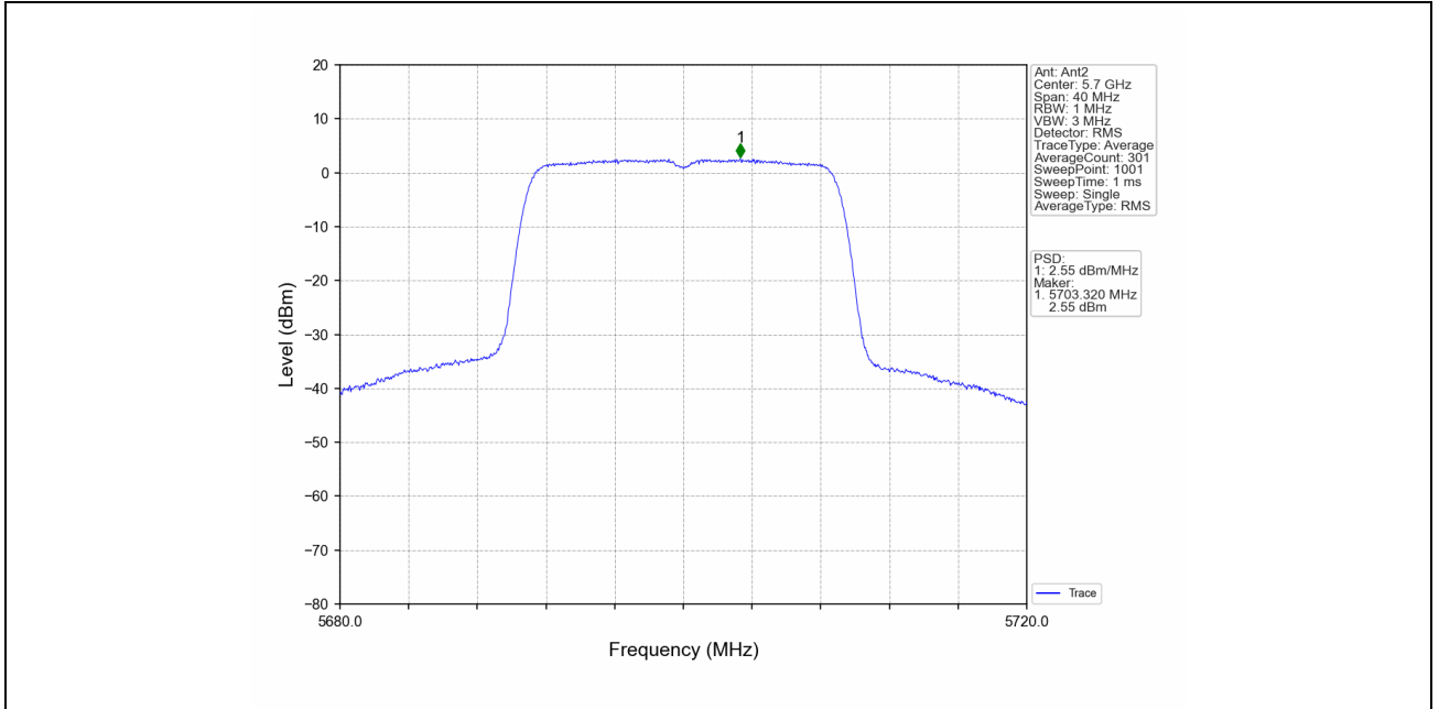
802.11ac(VHT20)_HCH_5700MHz_MIMO_NTNV
