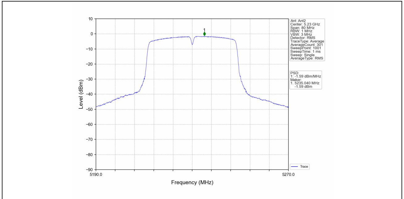
802.11ac(VHT40)_HCH_5230MHz_MIMO_NTNV
