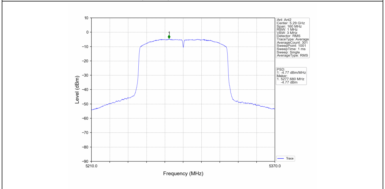
802.11ac(VHT80)_MCH_5290MHz_MIMO_NTNV
