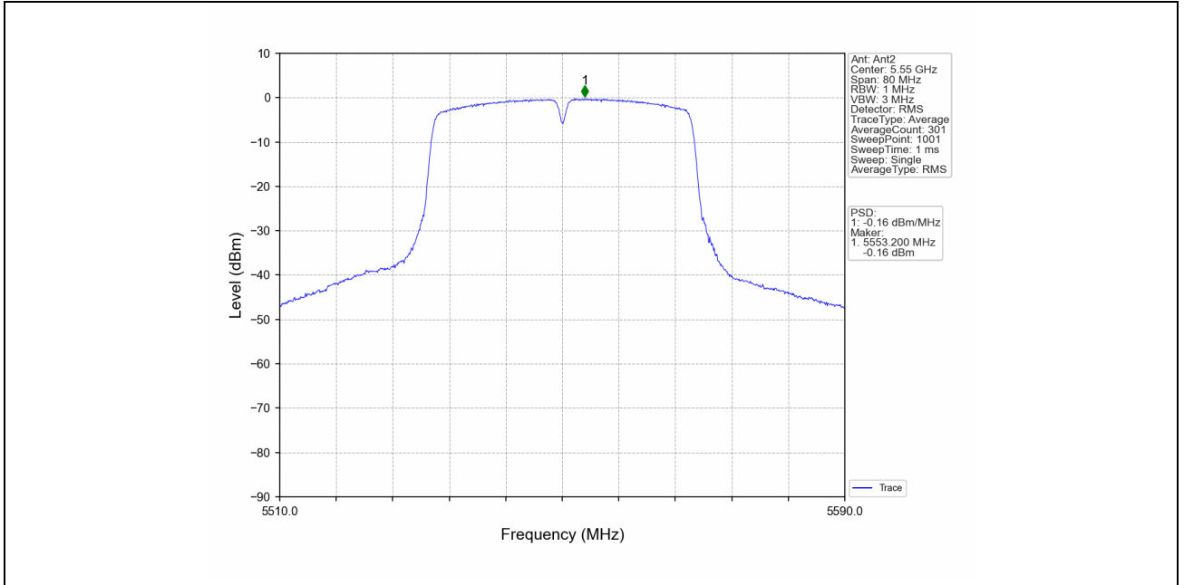
802.11ac(VHT40)_MCH_5550MHz_MIMO_NTNV
