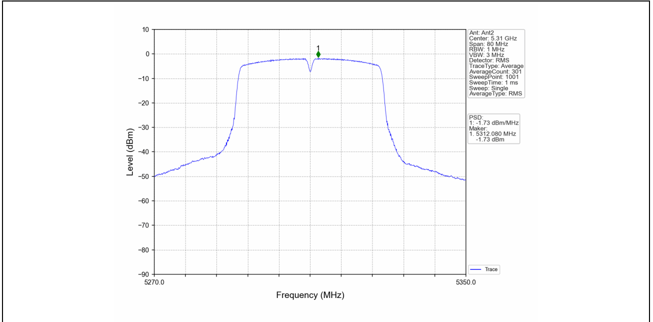
802.11ac(VHT40)_HCH_5310MHz_MIMO_NTNV
