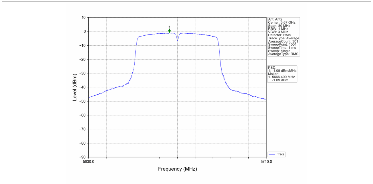
802.11ac(VHT40)_HCH_5670MHz_MIMO_NTNV
