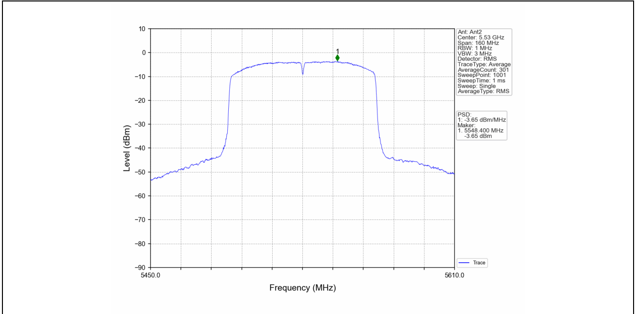
802.11ac(VHT80)_LCH_5530MHz_MIMO_NTNV
