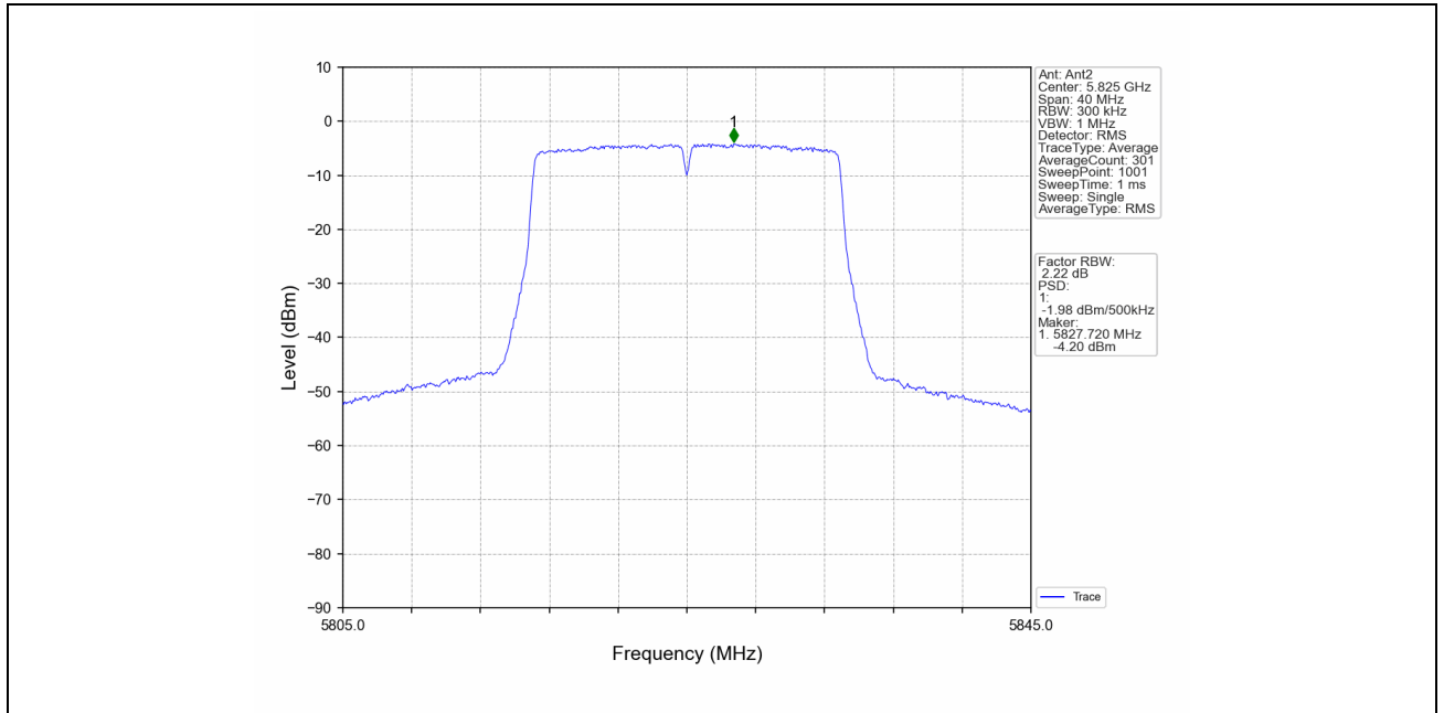
802.11ac(VHT20)_HCH_5825MHz_MIMO_NTNV
