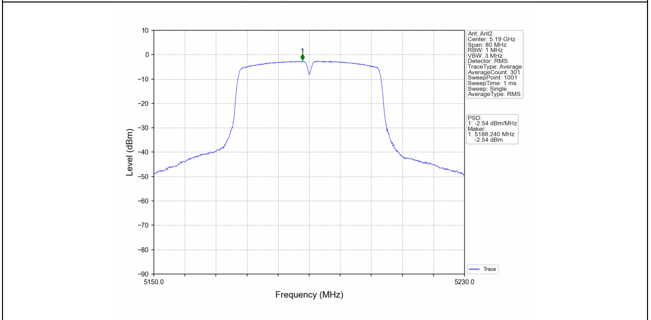
802.11ac(VHT40)_LCH_5190MHz_MIMO_NTNV
