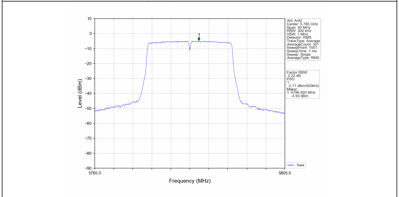
802.11ac(VHT20)_MCH_5785MHz_MIMO_NTNV
