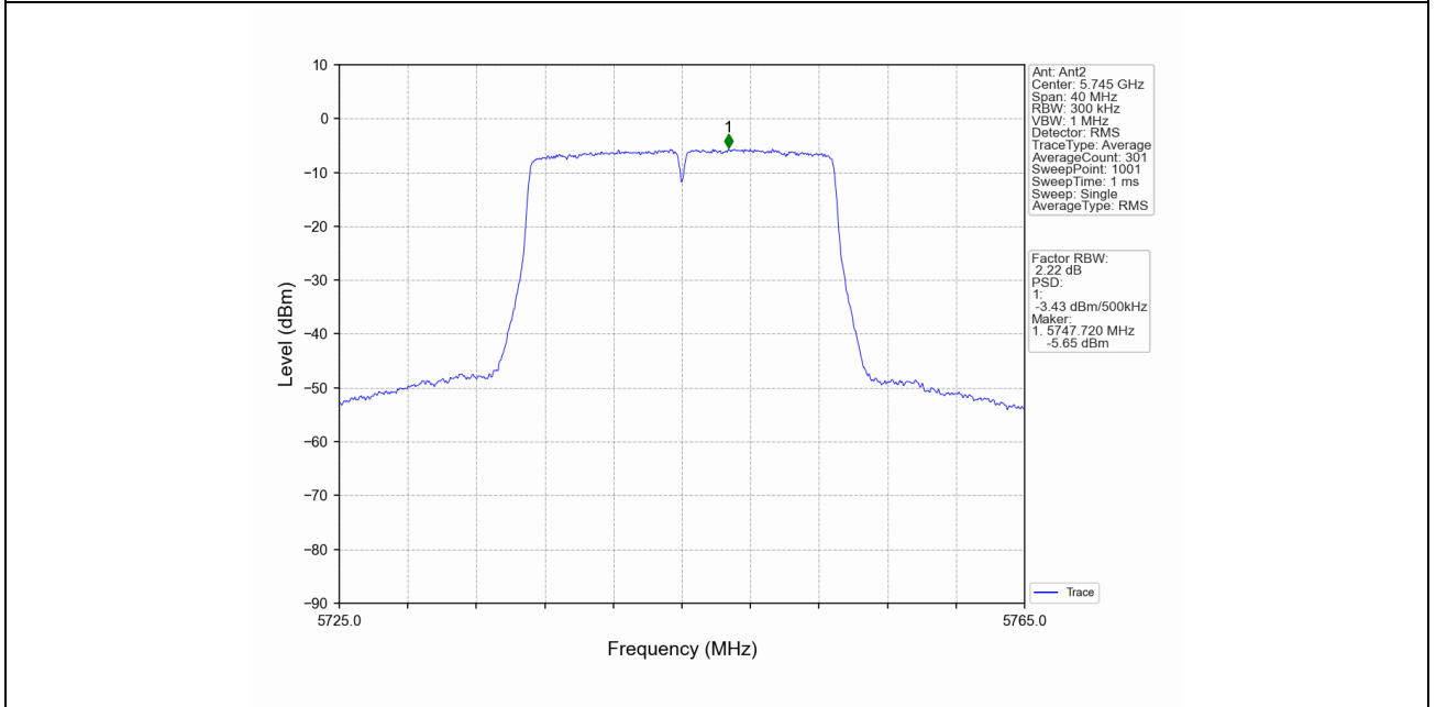
802.11n(HT20)_LCH_5745MHz_MIMO_NTNV
