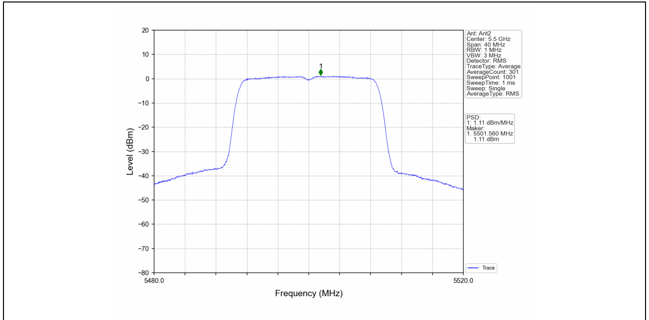
802.11ac(VHT20)_LCH_5500MHz_MIMO_NTNV
