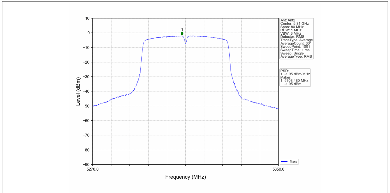
802.11n(HT40)_HCH_5310MHz_MIMO_NTNV
