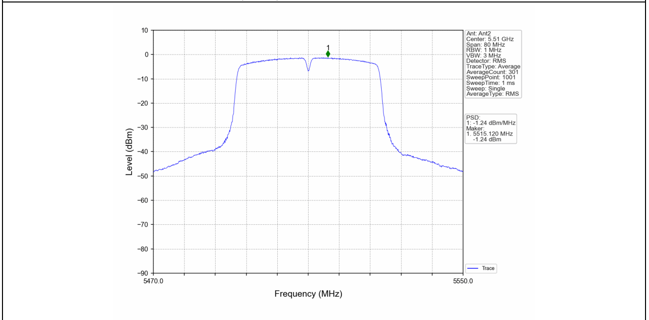
802.11n(HT40)_LCH_5510MHz_MIMO_NTNV
