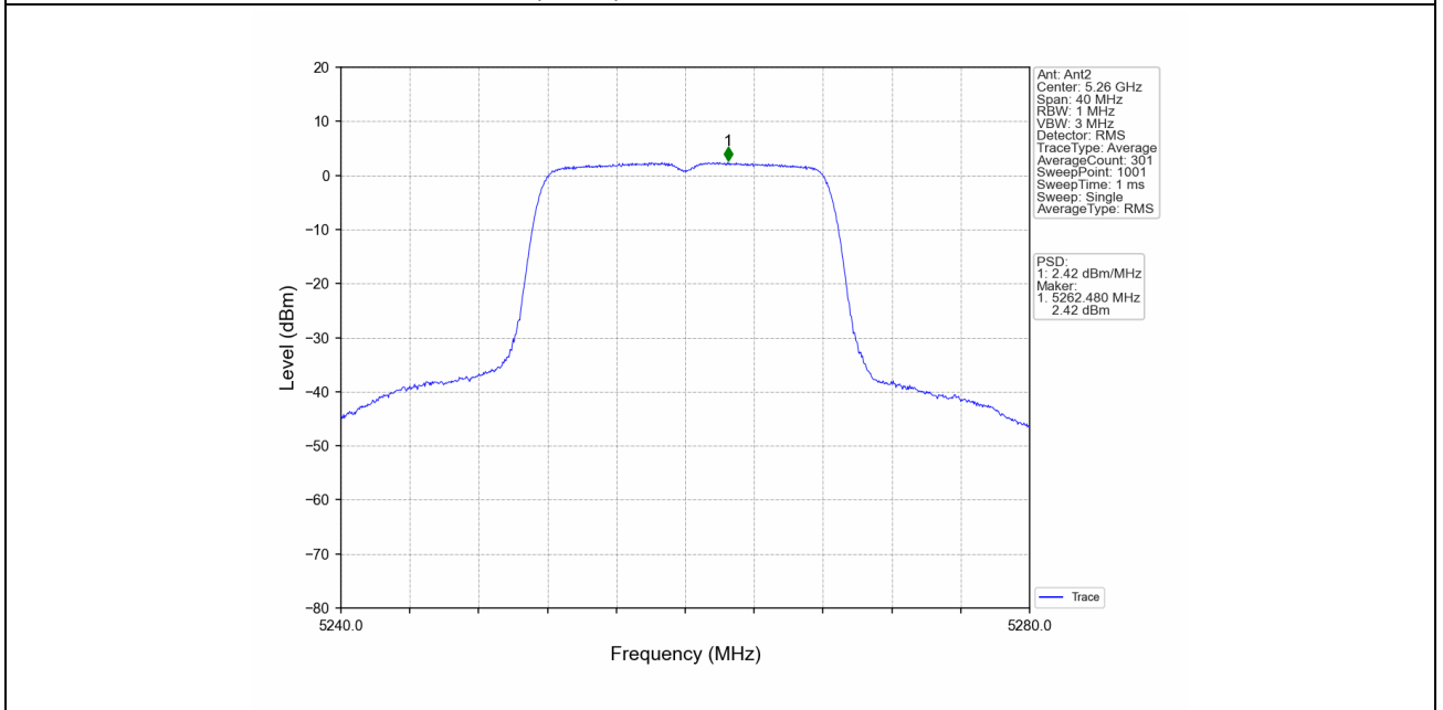
802.11n(HT20)_LCH_5260MHz_MIMO_NTNV
