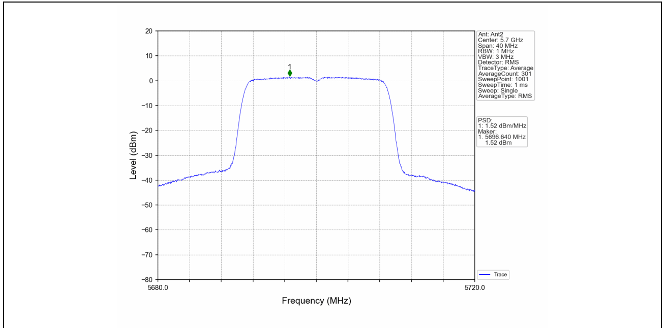
802.11n(HT20)_HCH_5700MHz_MIMO_NTNV
