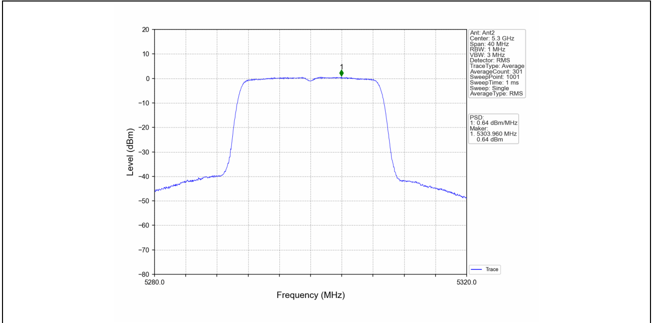
802.11ac(VHT20)_MCH_5300MHz_MIMO_NTNV
