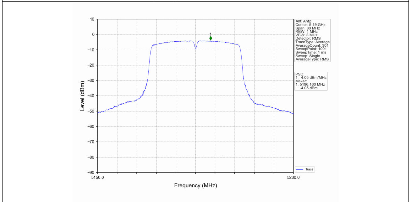
802.11n(HT40)_LCH_5190MHz_MIMO_NTNV
