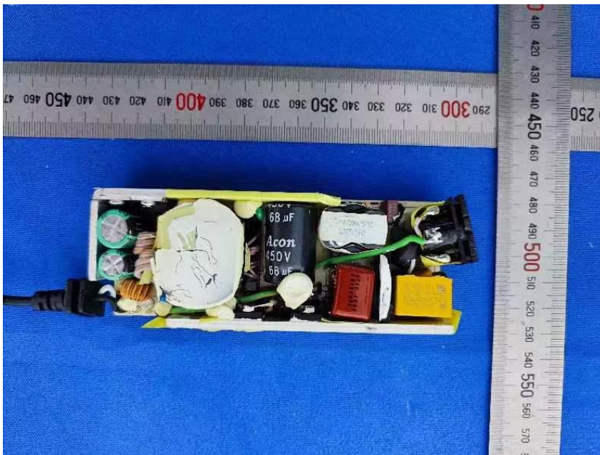
Adapter FSP090-DIEBN2
