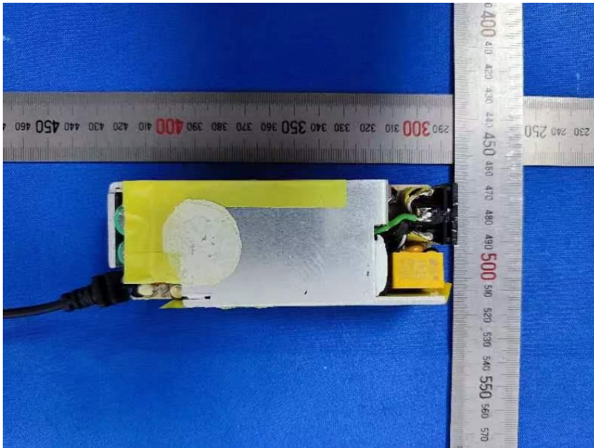
Adapter FSP090-DIEBN2
