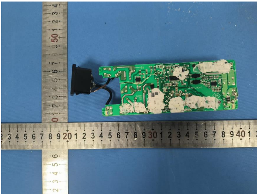
Adapter DPS-90AB-3
