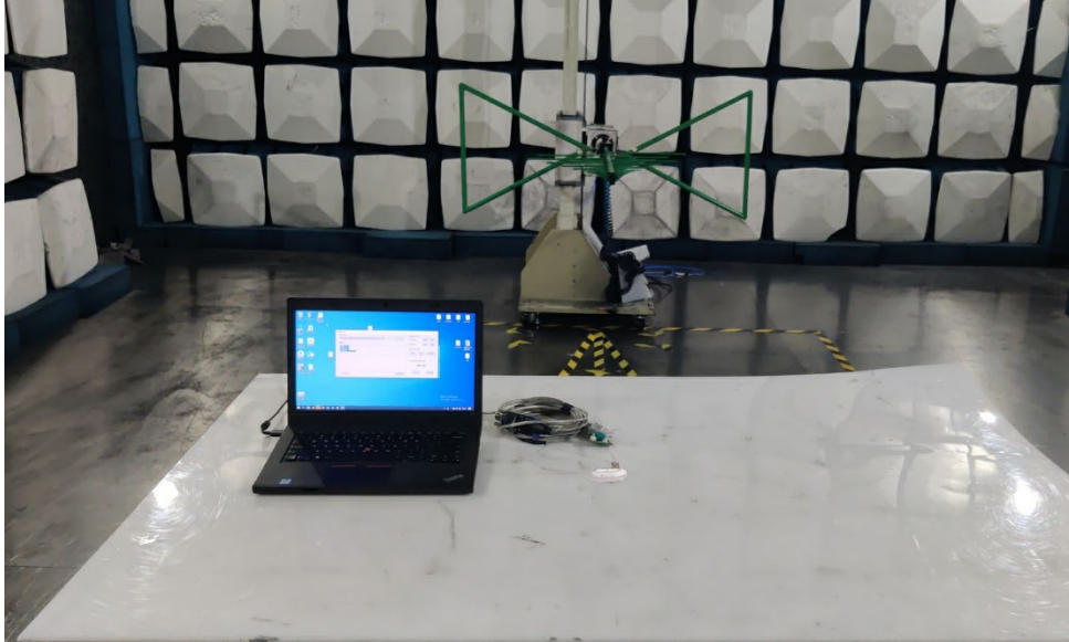
Radiated Emissions below 1GHz
