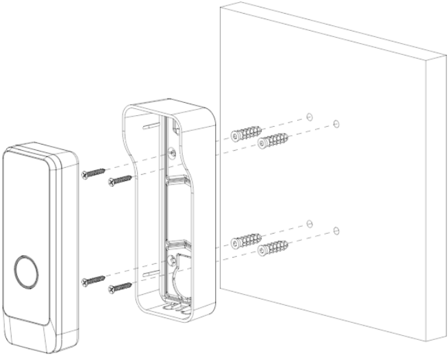
Figure 2-8 Installation
