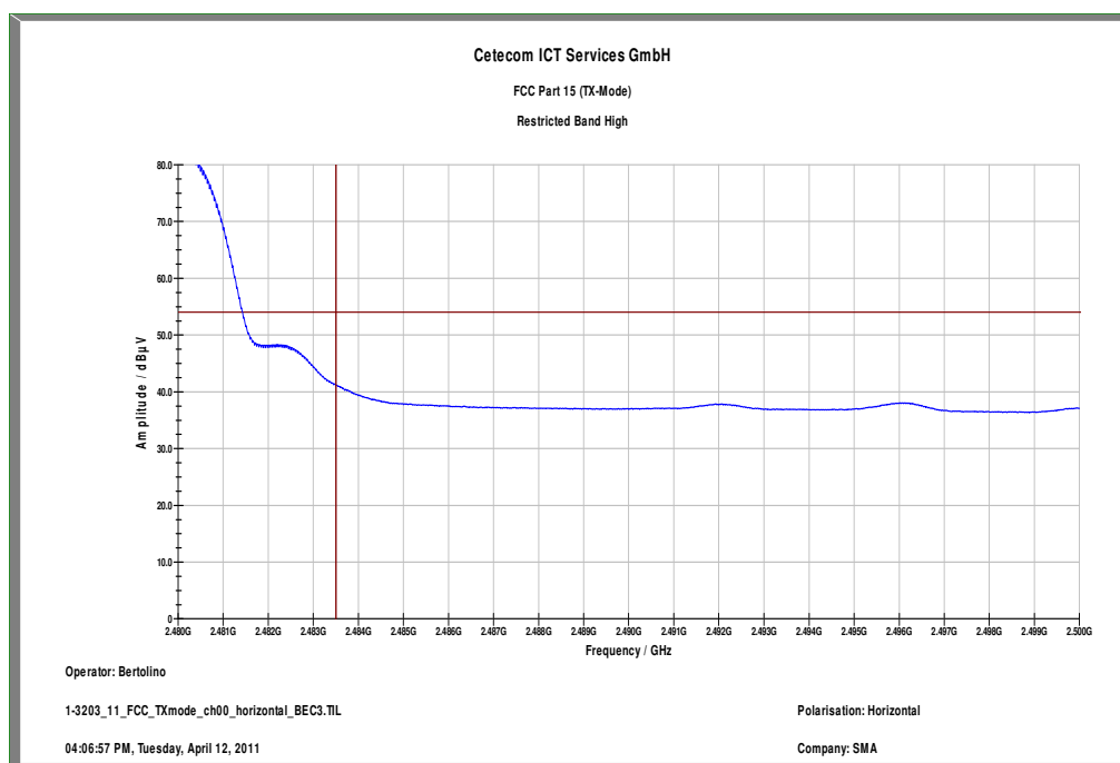
Plot 12: Upper restricted band, 8DPSK, horizontal polarization
