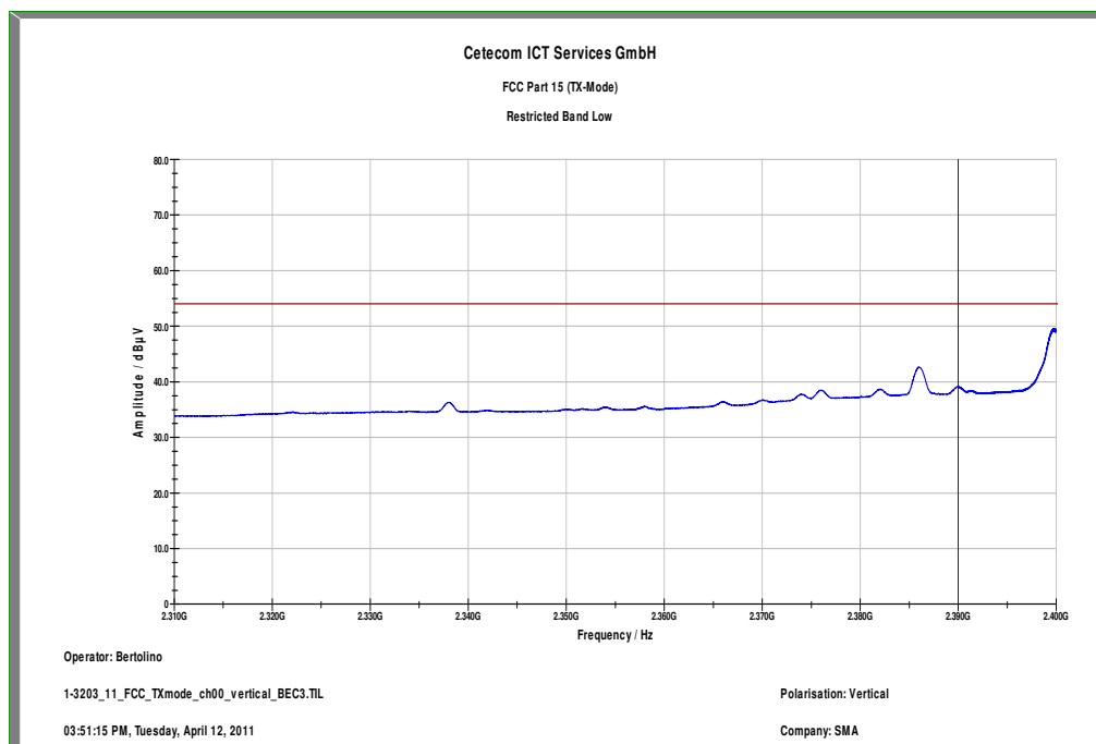
Plot 9: Lower restricted band, 8DPSK, vertical polarization
