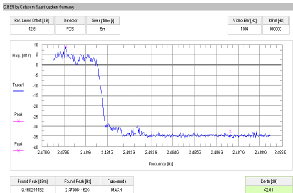
Plot 10: Upper band edge – hopping on / 8DPSK (conducted)
