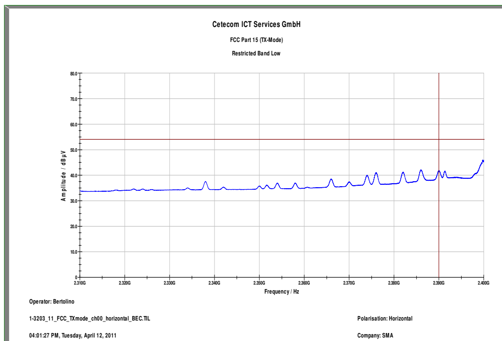
Plot 3: Lower restricted band, GFSK, horizontal polarization
