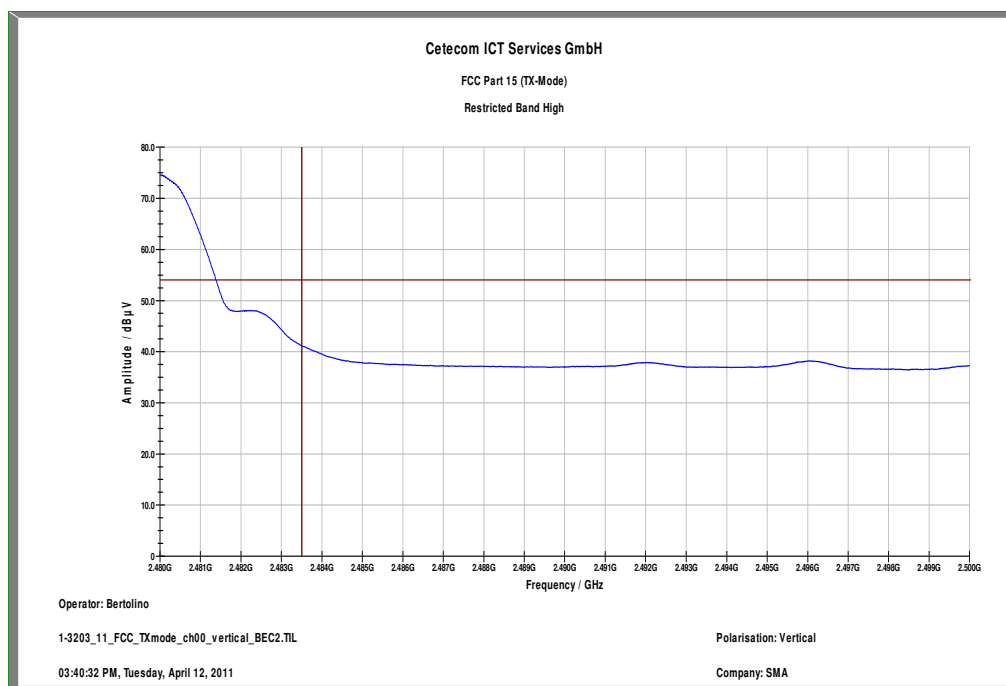
Plot 6: Upper restricted band, Pi/4 DQPSK, vertical polarization
