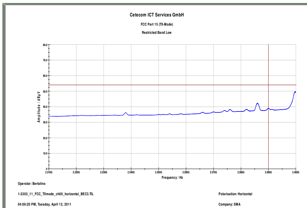
Plot 11: Lower restricted band, 8DPSK, horizontal polarization
