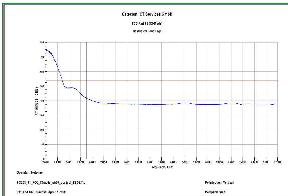
Plot 10: Upper restricted band, 8DPSK, vertical polarization
