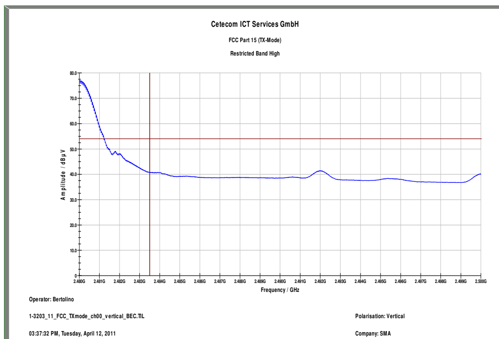
Plot 2: Upper restricted band, GFSK, vertical polarization
