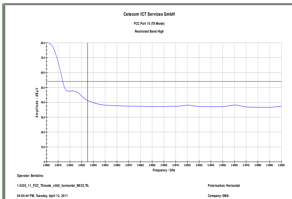
Plot 8: Upper restricted band, Pi/4 DQPSK, horizontal polarization
