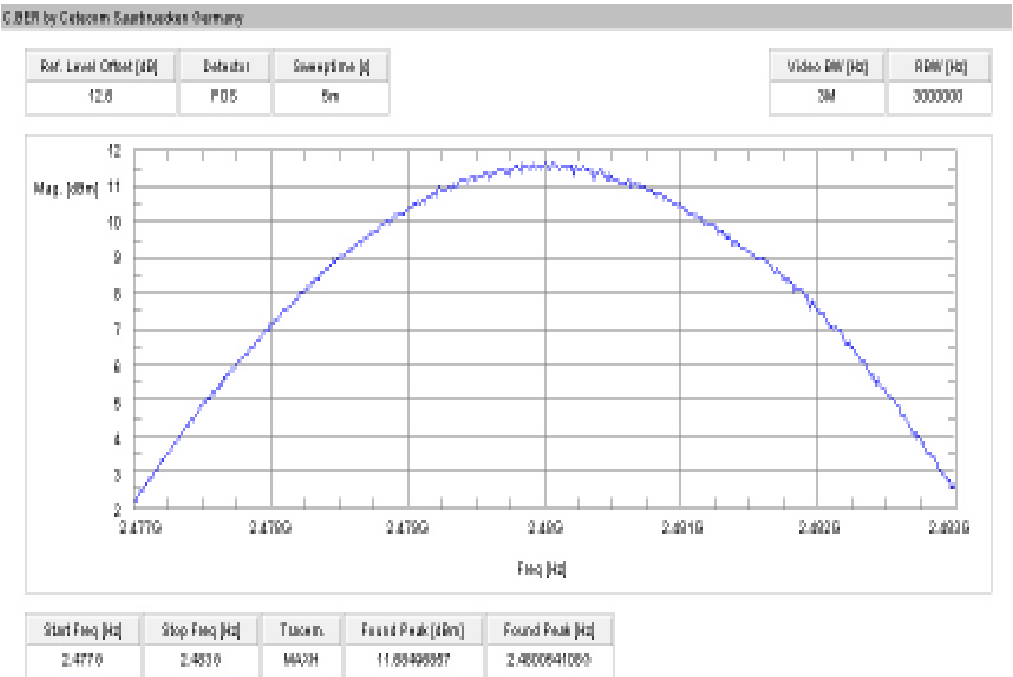
Plot 9: Channel 78 / 8DPSK (conducted)
