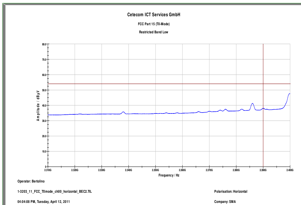
Plot 7: Lower restricted band, Pi/4 DQPSK, horizontal polarization
