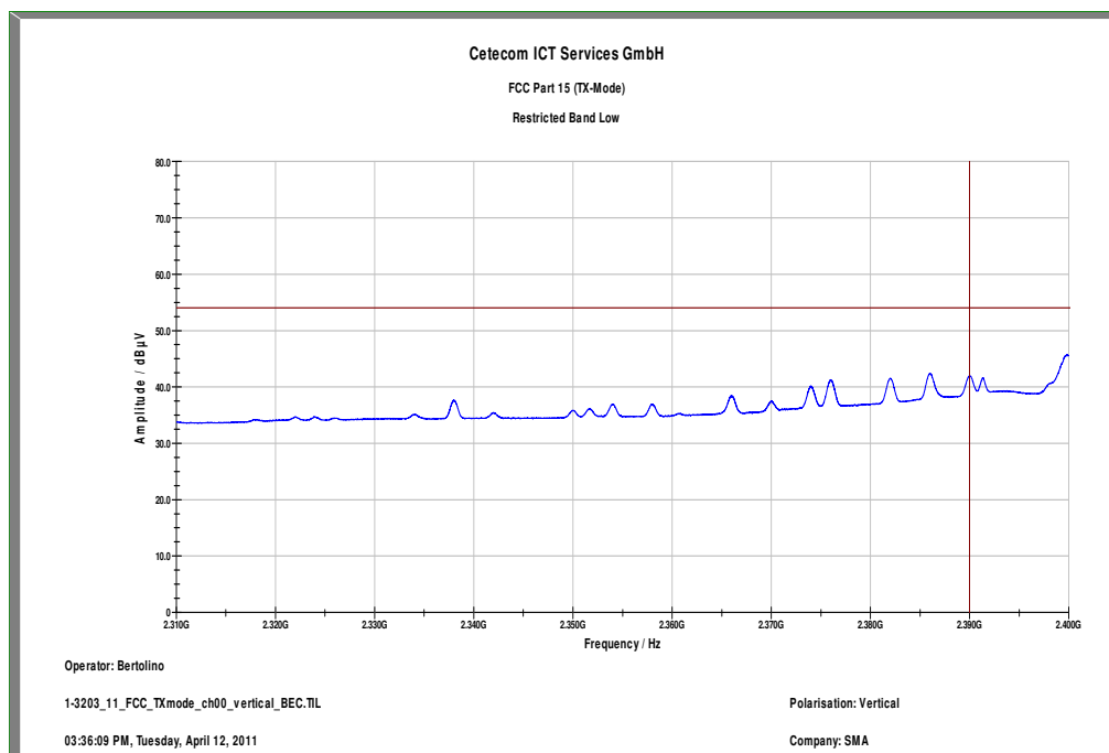
Plot 1: Lower restricted band, GFSK, vertical polarization
