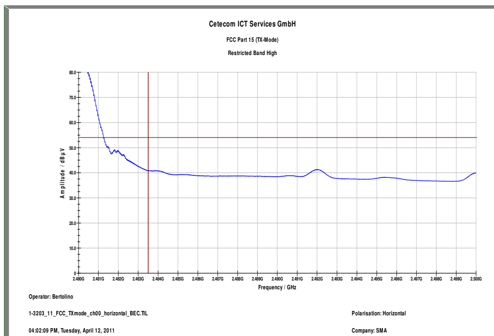
Plot 4: Upper restricted band, GFSK, horizontal polarization
