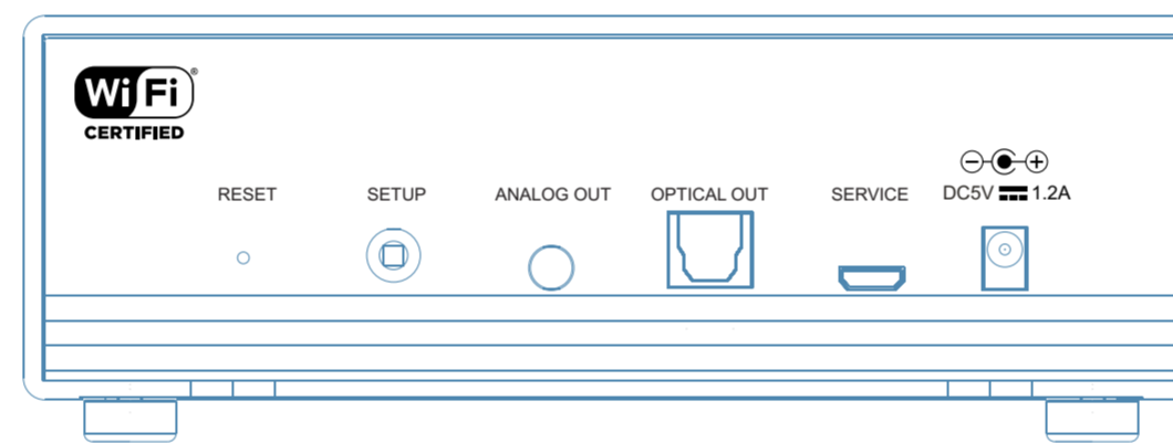
MT2 Rear Panel
