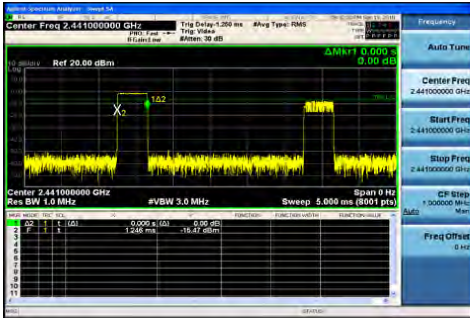
Dwell Time_DH1_2441
