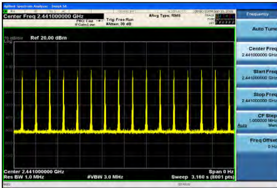
Dwell Time_3DH5_2441
