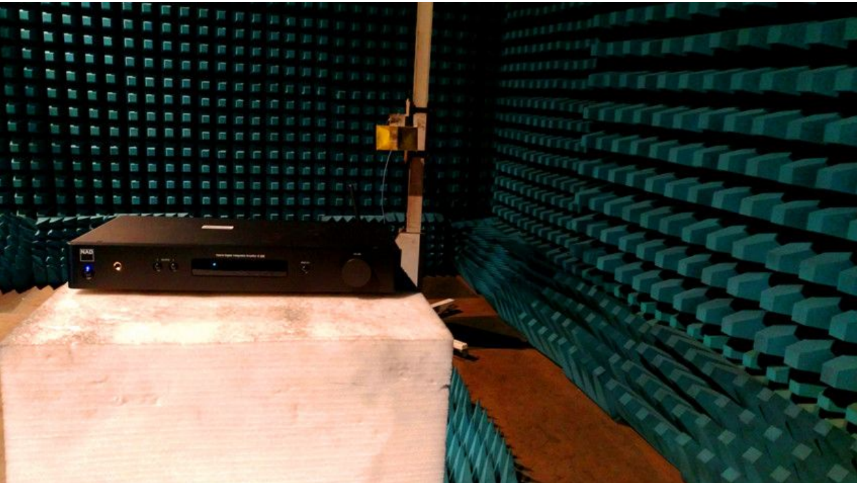
Above 1GHz
