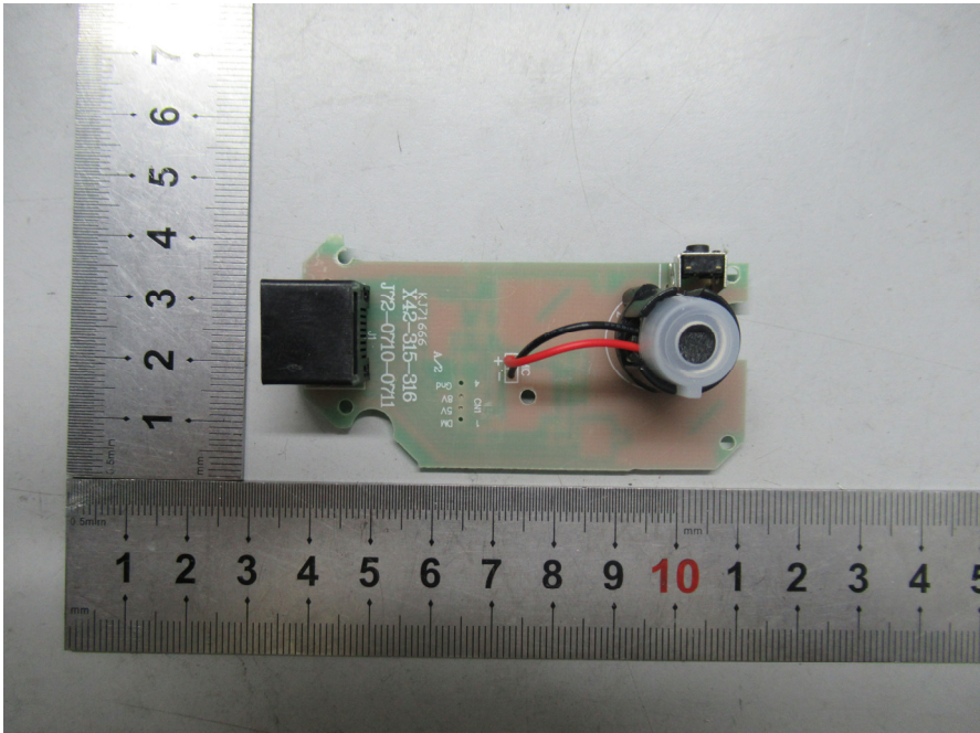
EUT (Microphone) – PCB3 Bottom View
