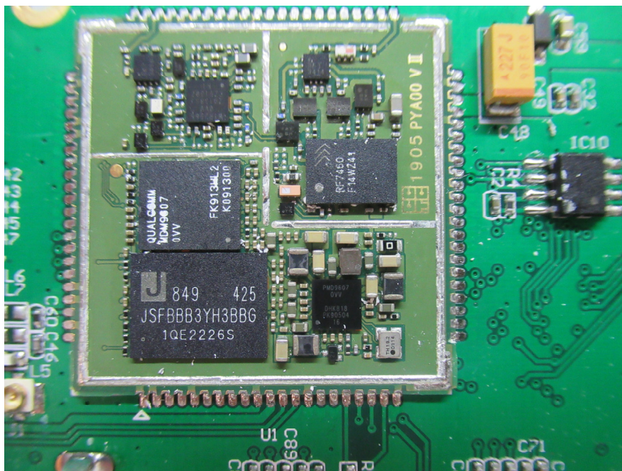
EUT(POC Mobile Radio) –PCB1 Bottom Chip View
