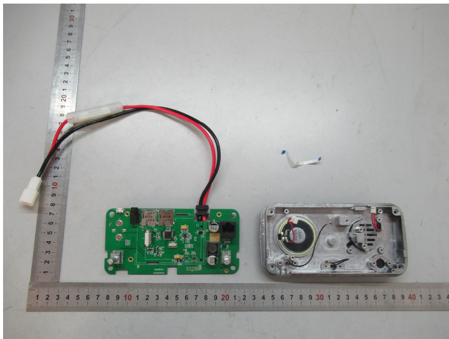
EUT(POC Mobile Radio) – Cover off View-2
