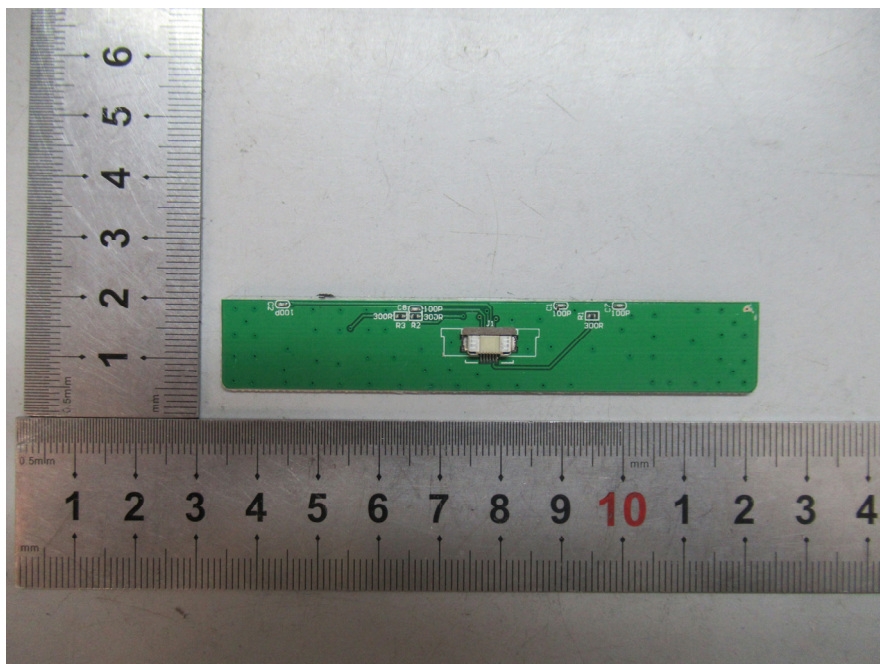
EUT(POC Mobile Radio) – PCB2 Top View
