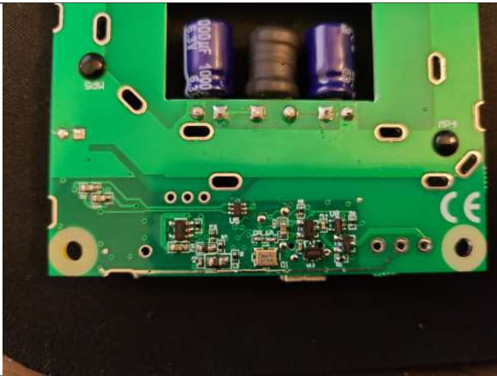
Component Placement-Back
