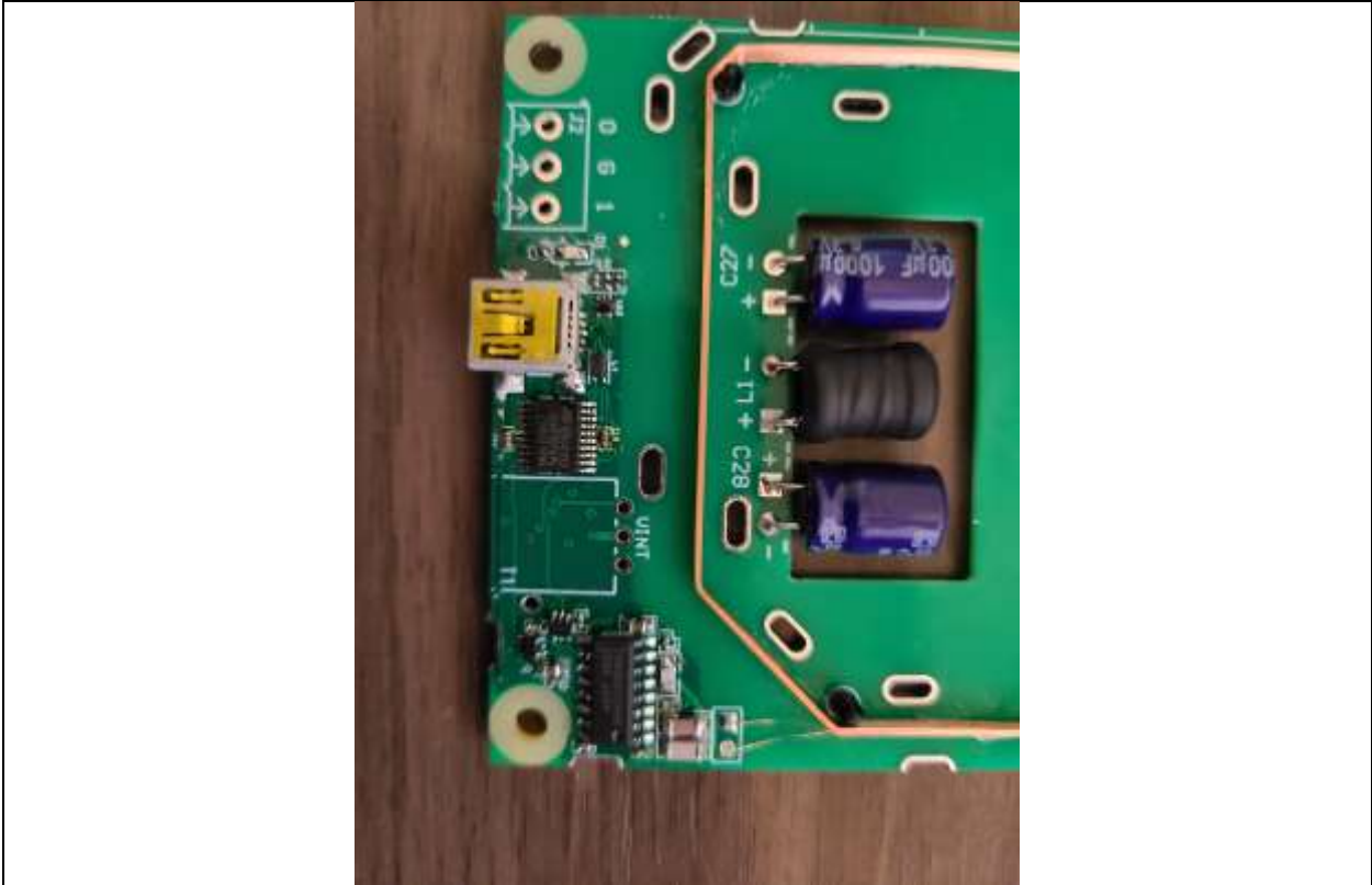
Component Placement-Front
