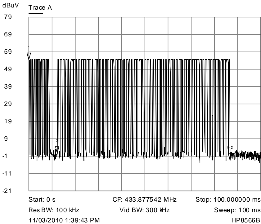
Trace A 100 ms plot - 3-2 shows length of THOP + TFIX
