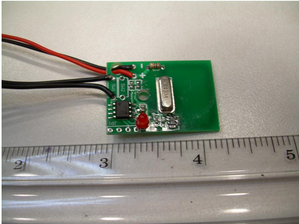
Photograph 4 – Front View of EUT
