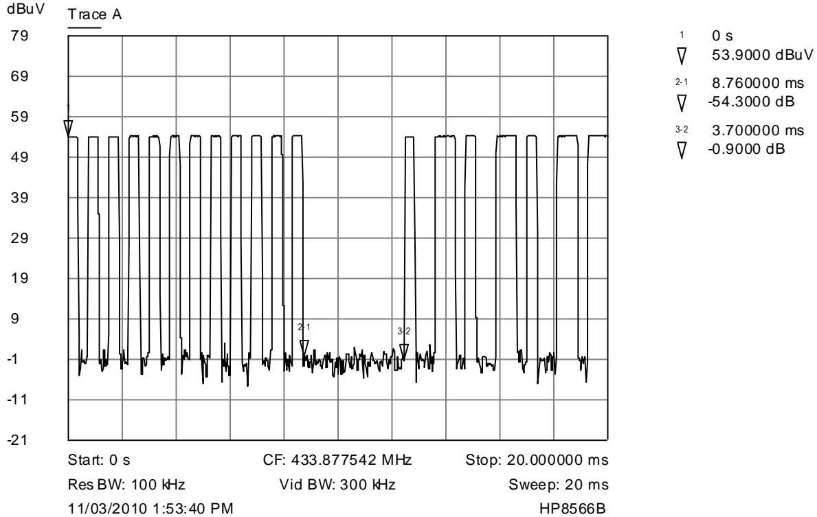
Trace A TP and TH timing
