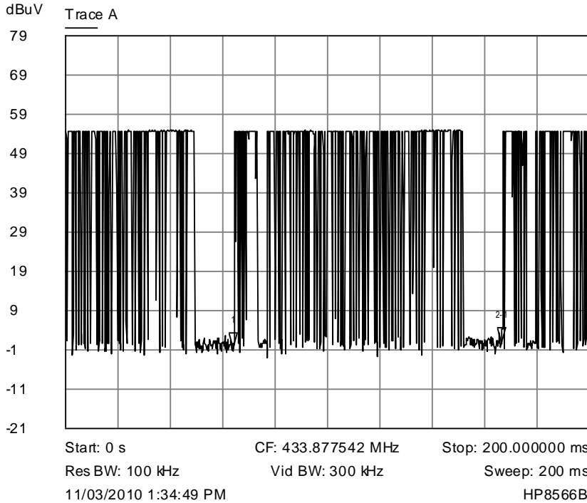
Trace A 200 ms plot
