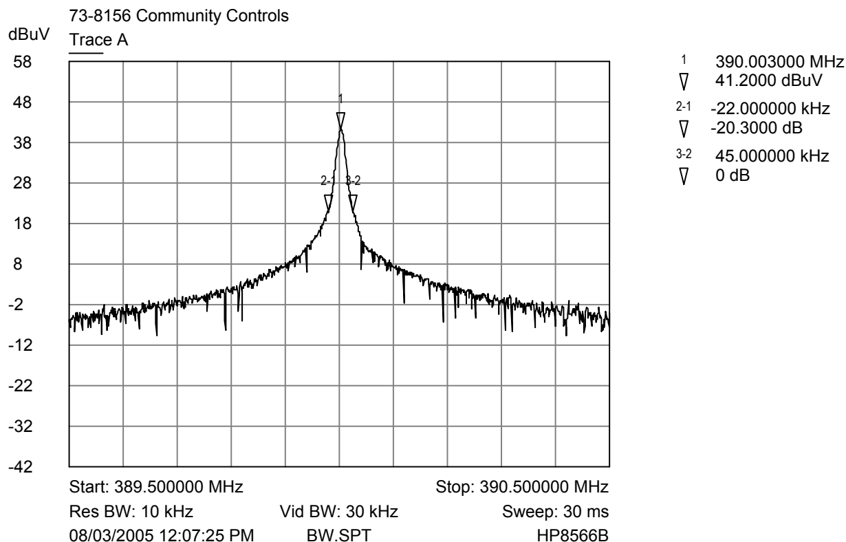
TRACOMFIR611K Bandwidth Plot
