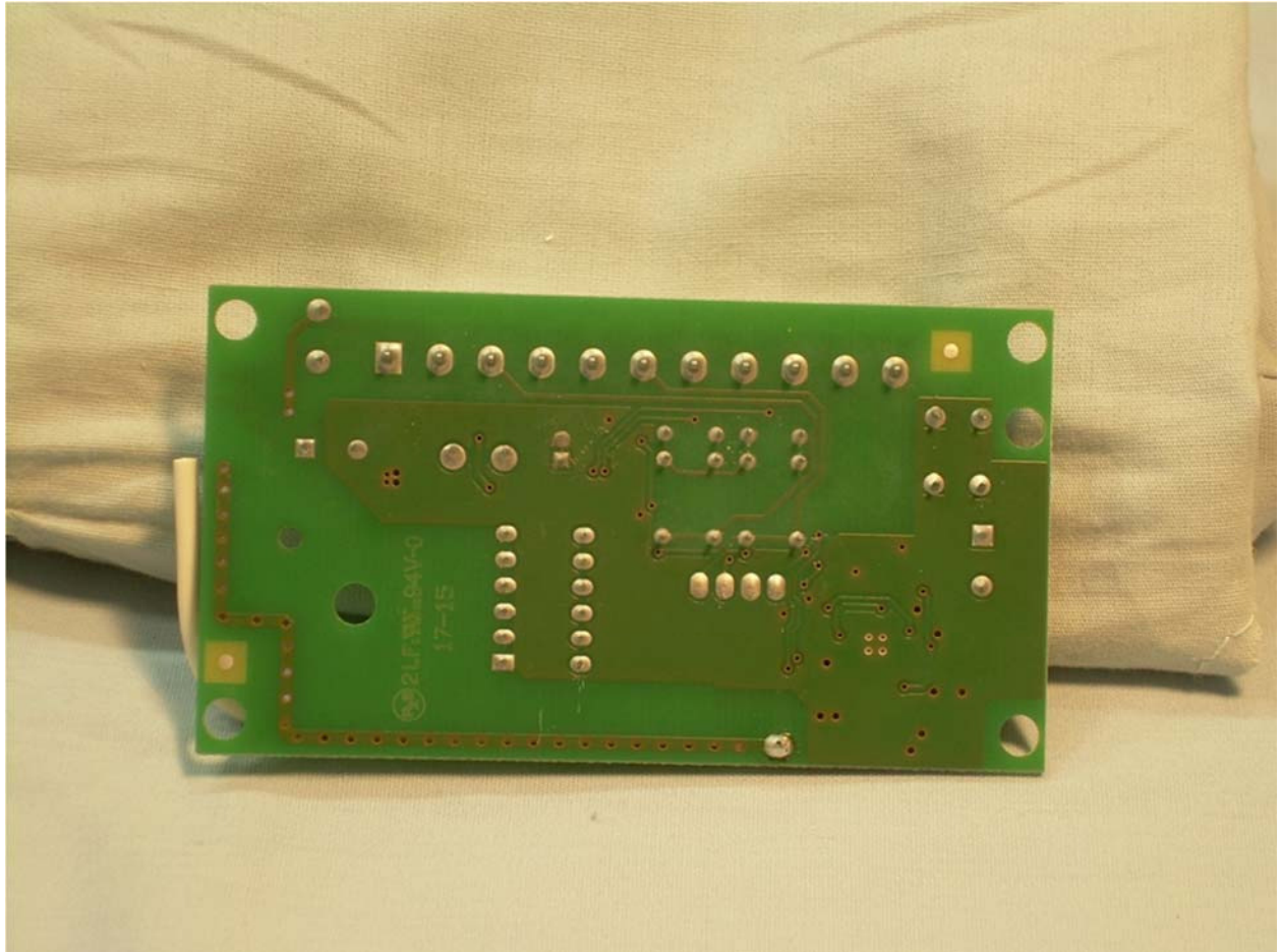
View of the Trace Side of the RCO0900
