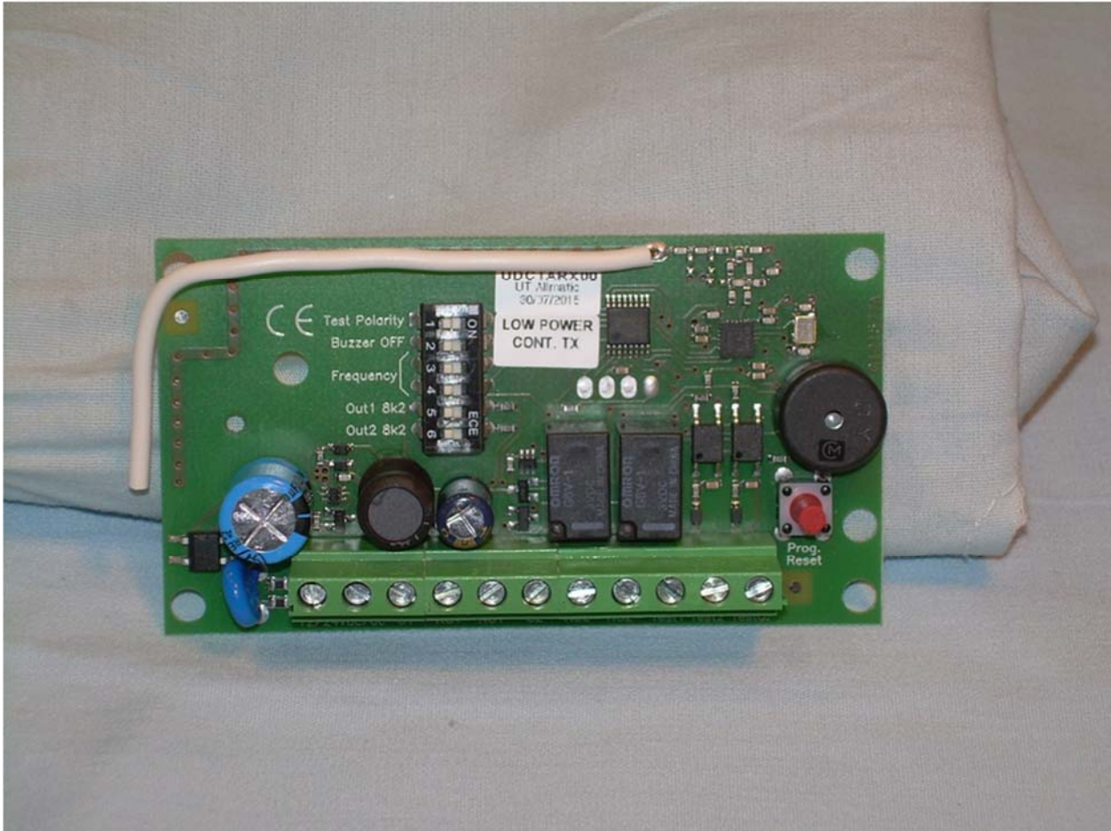
View of the Component Side of the RCOO900
