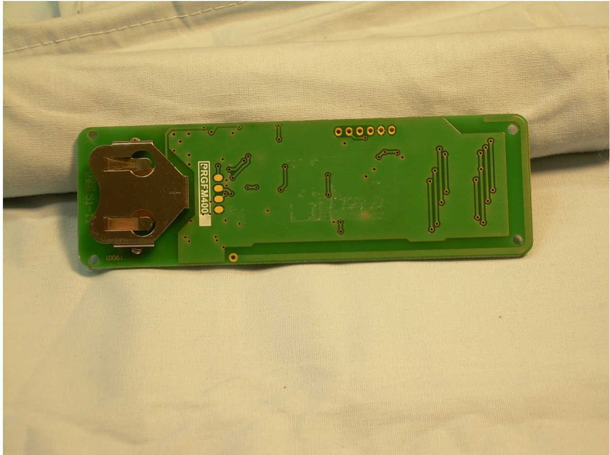
Photograph 8 – View of the Bottom Side of the PCB
