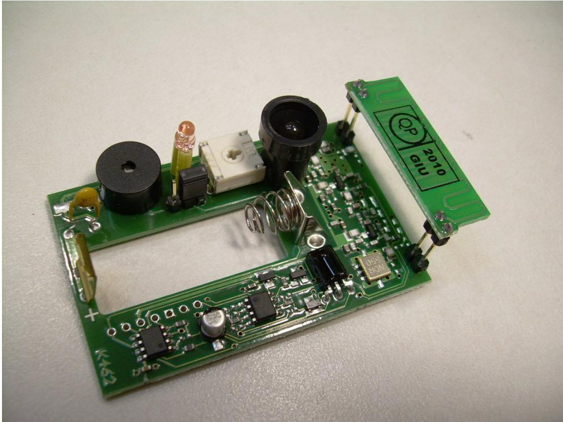
Photograph 7 – Top View of the PCB
