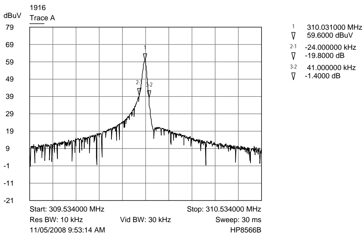
EMP310LID21V Bandwidth Plot
