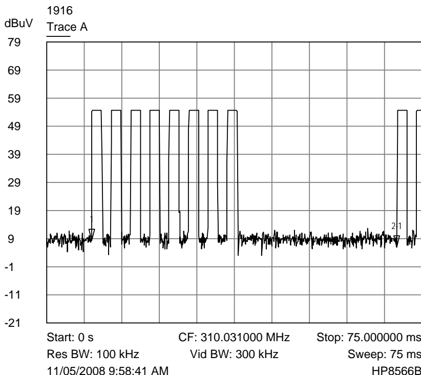
Trace A 75 ms pulse train plot
