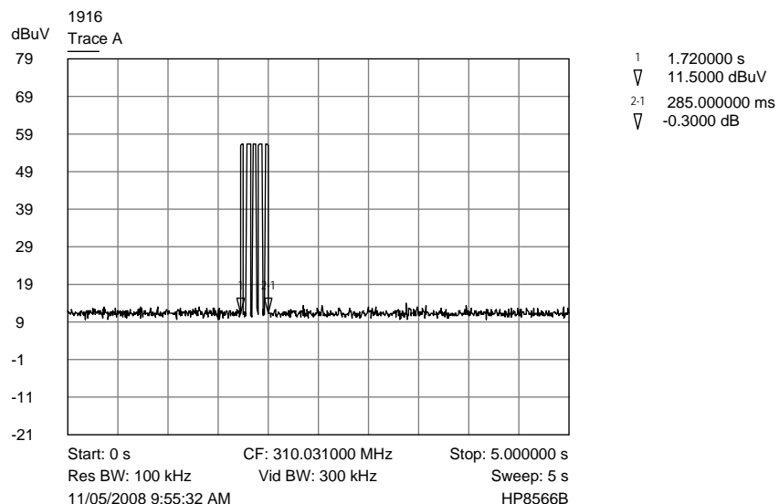
Trace A Button pressed to transmit and then released
