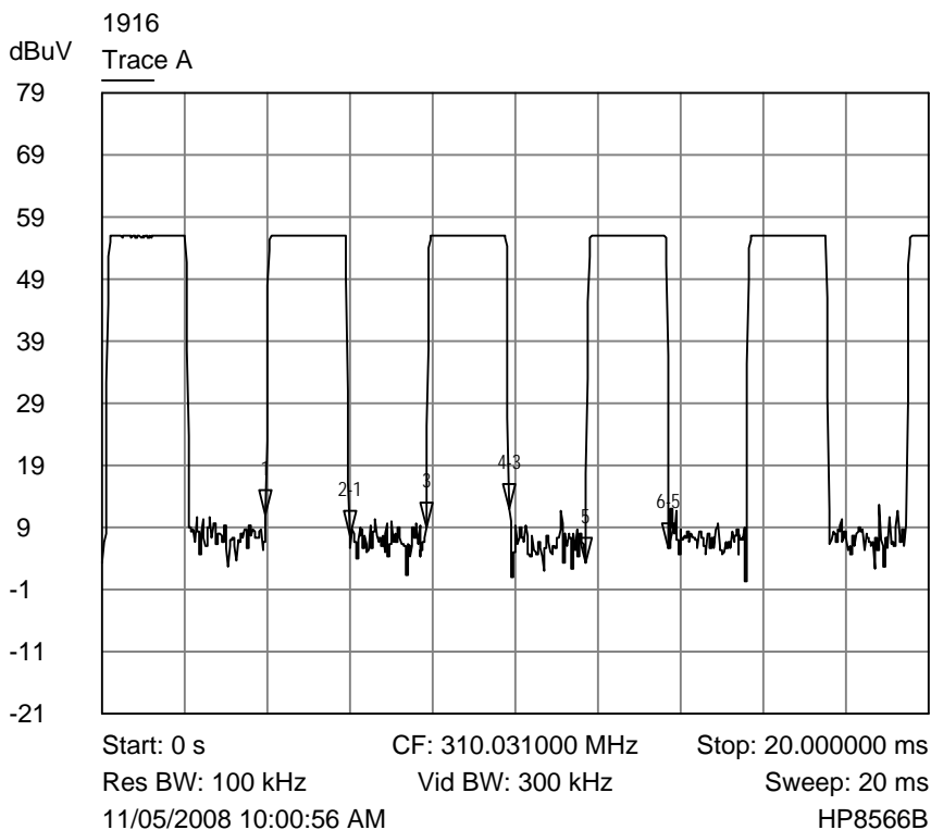
Trace A 20 ms pulse train plot
