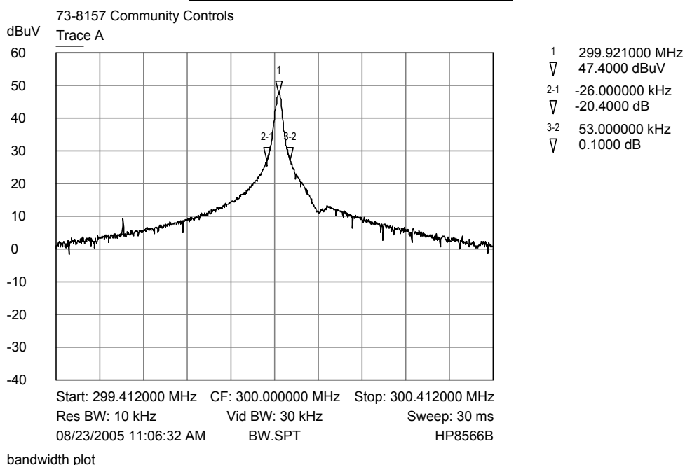
CCS3001BV Bandwidth Plot
