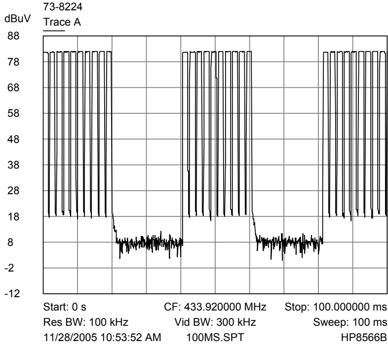
100ms plot to show pulse trains
