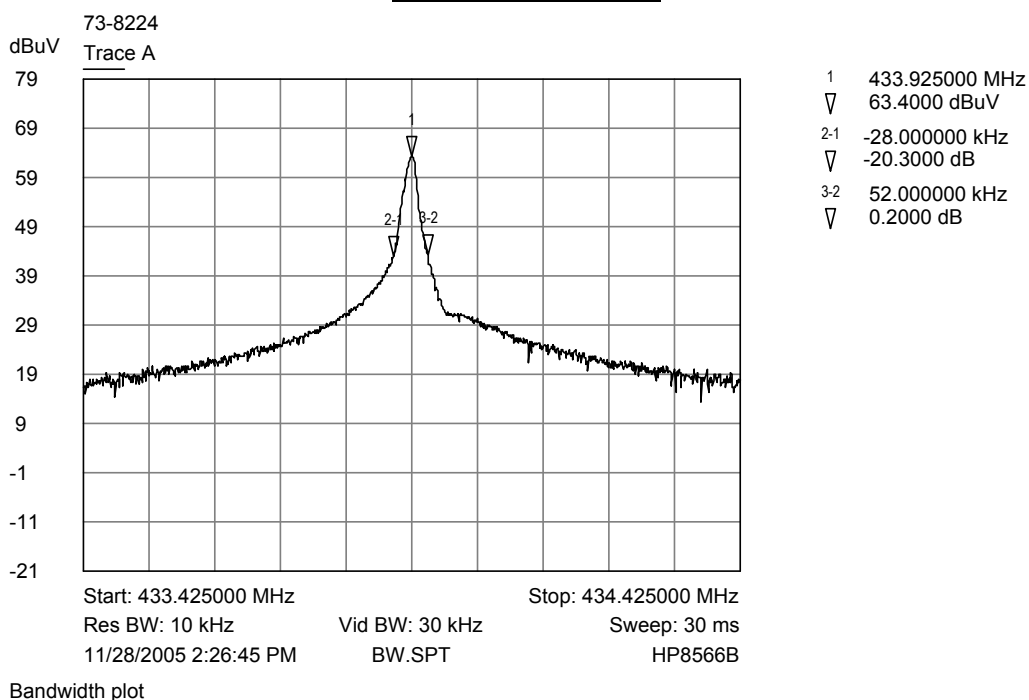
Bandwidth Plot
