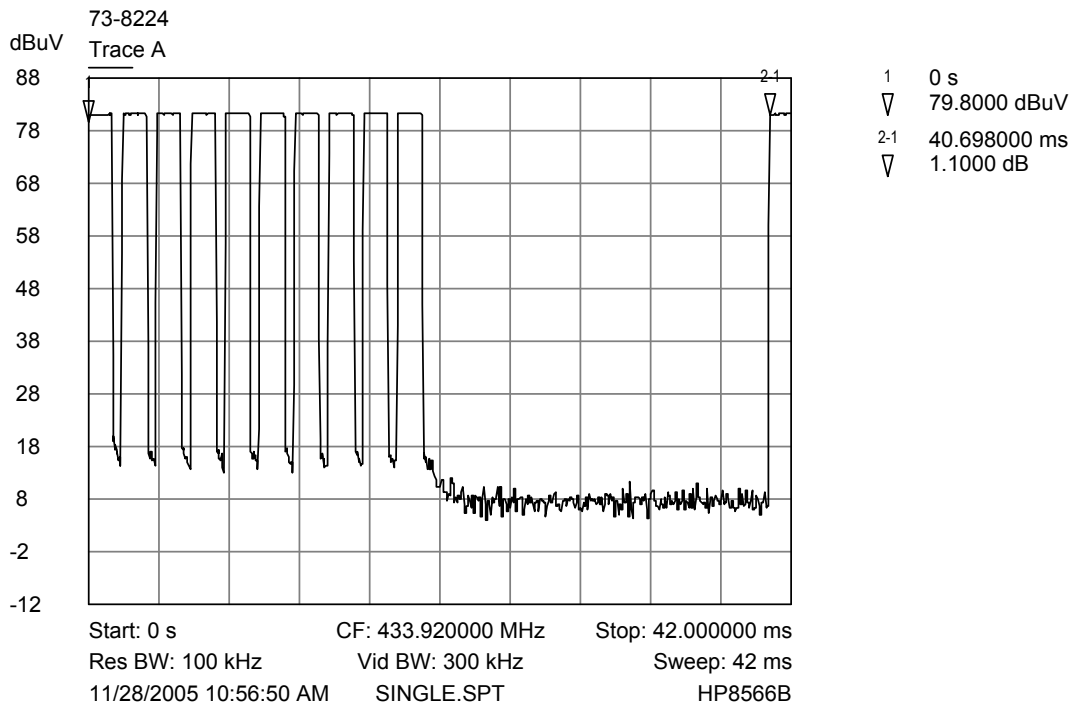
Single pulse train plot
