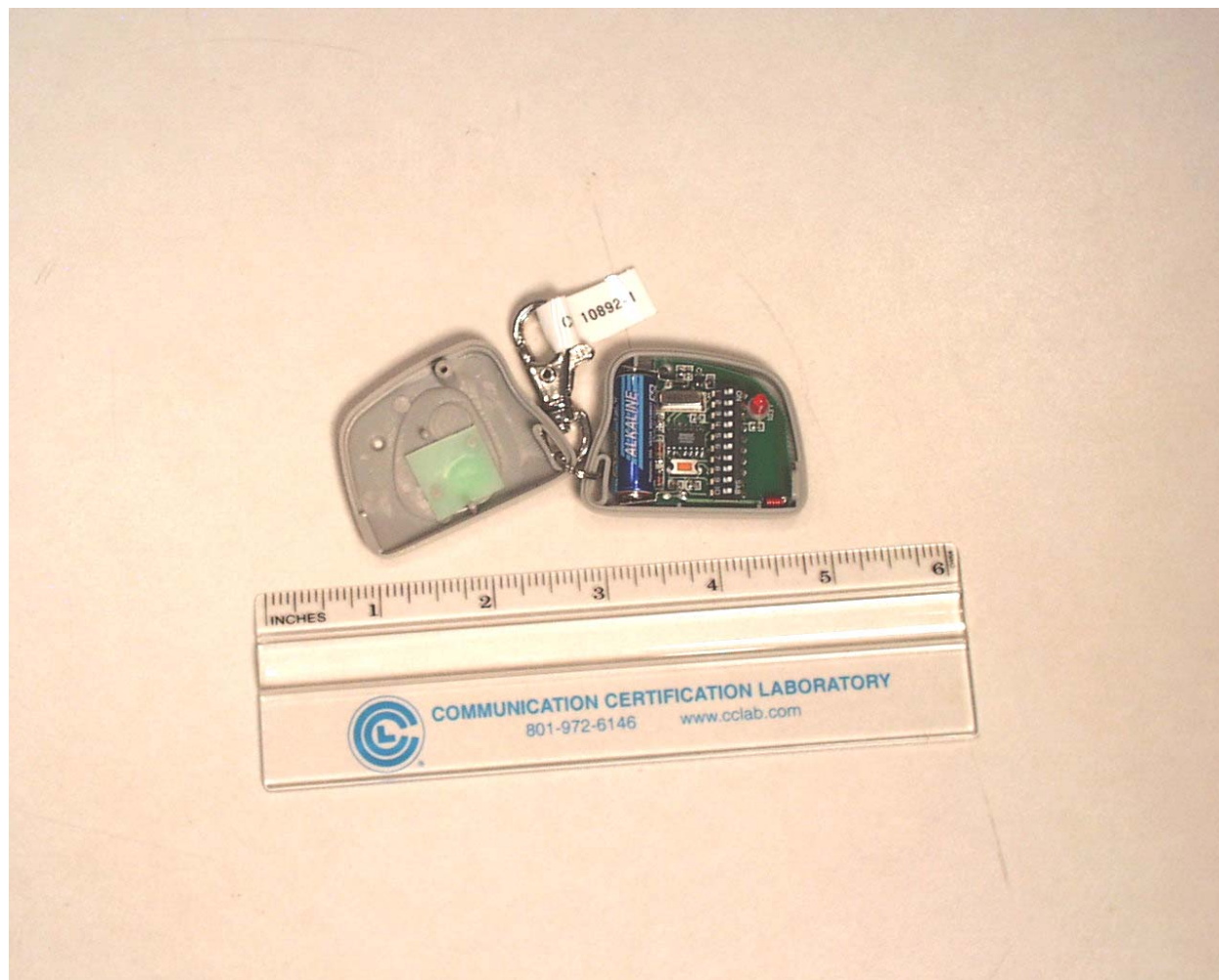
View of the EUT with the Case Opened
