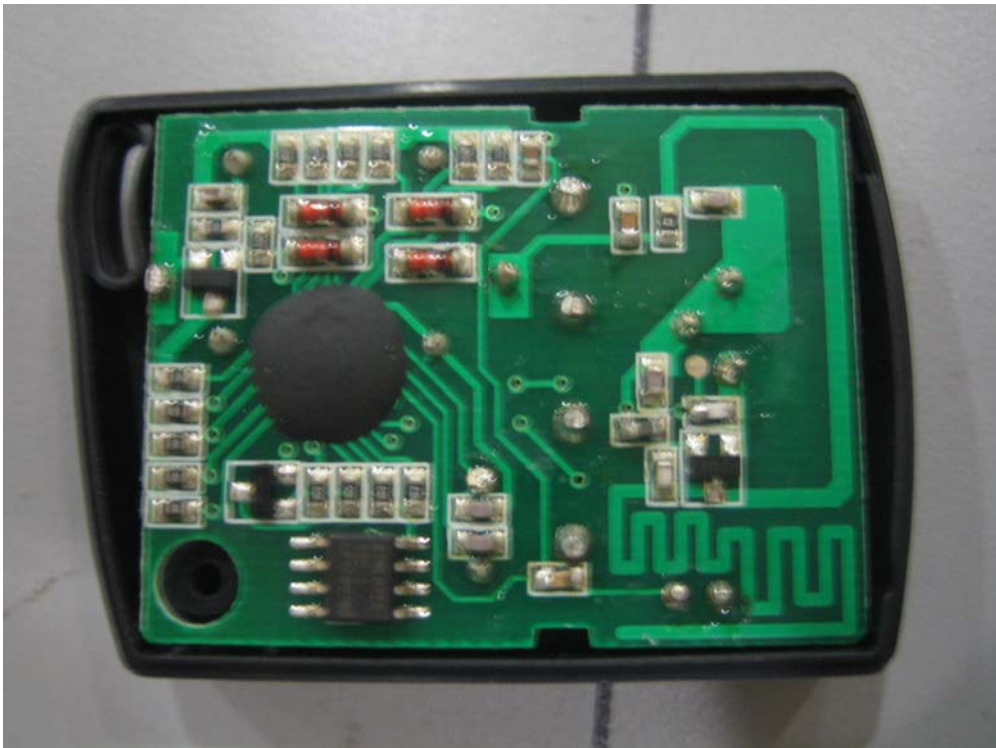
Front View (CC-601)
