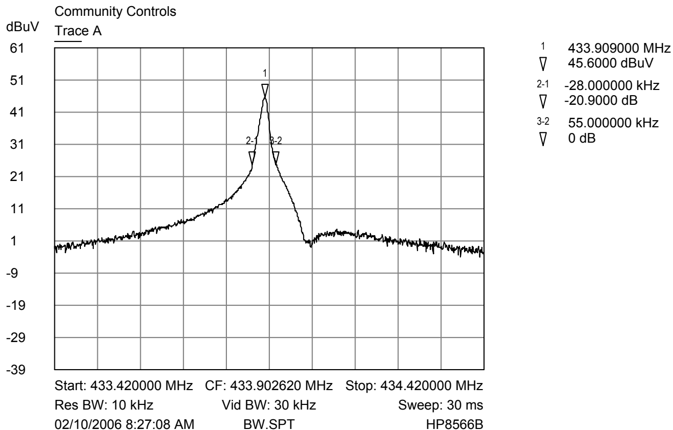
Bandwidth Plot
